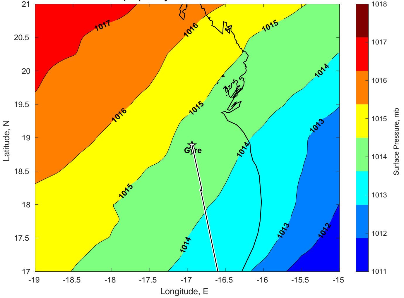
Surface Pressure (mb) for Gyre at 20-Mar-2025 00:00:00
