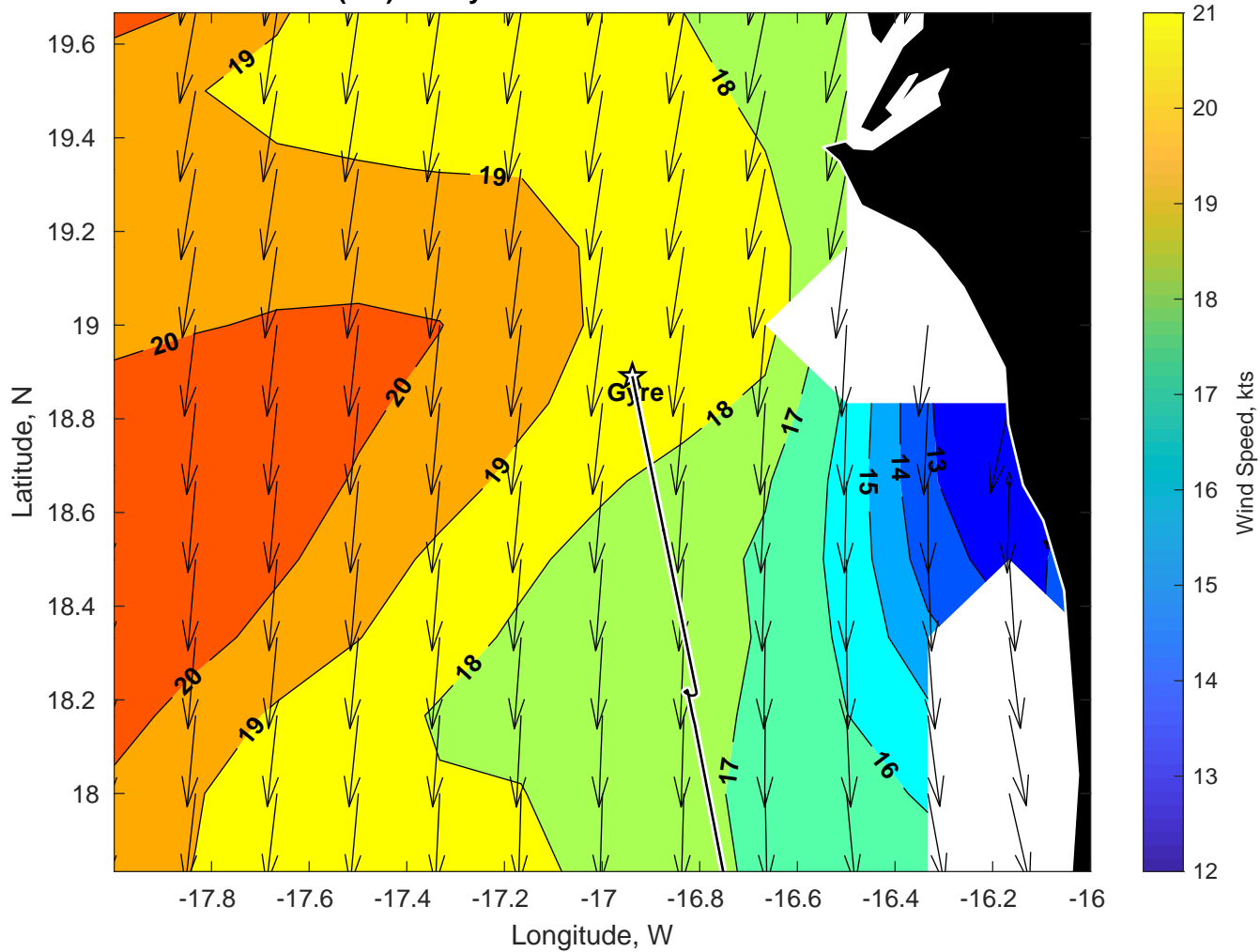
Winds (kts) for Gyre at 19-Mar-2025 09:00:00
