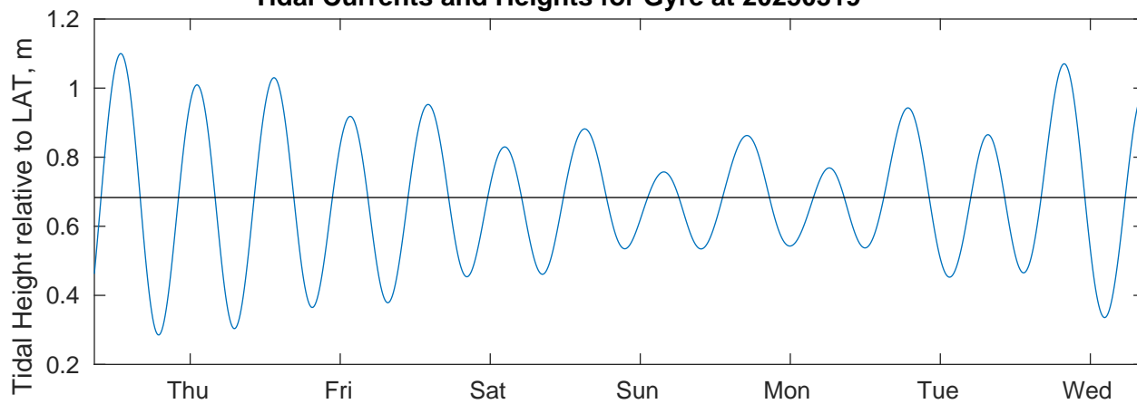
Tidal Currents and Heights for Gyre at 20250319
