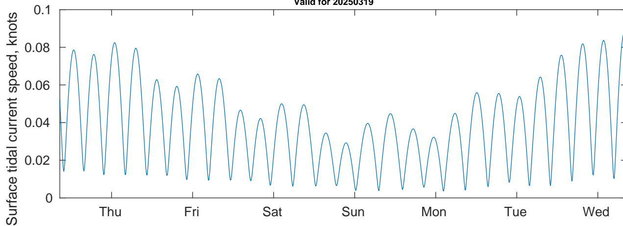
Tidal Currents and Heights for Gyre at 20250319
