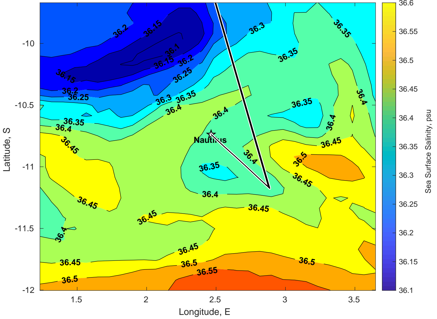
Surface Salinity for Nautilus at 18-Mar-2025 00:00:00
