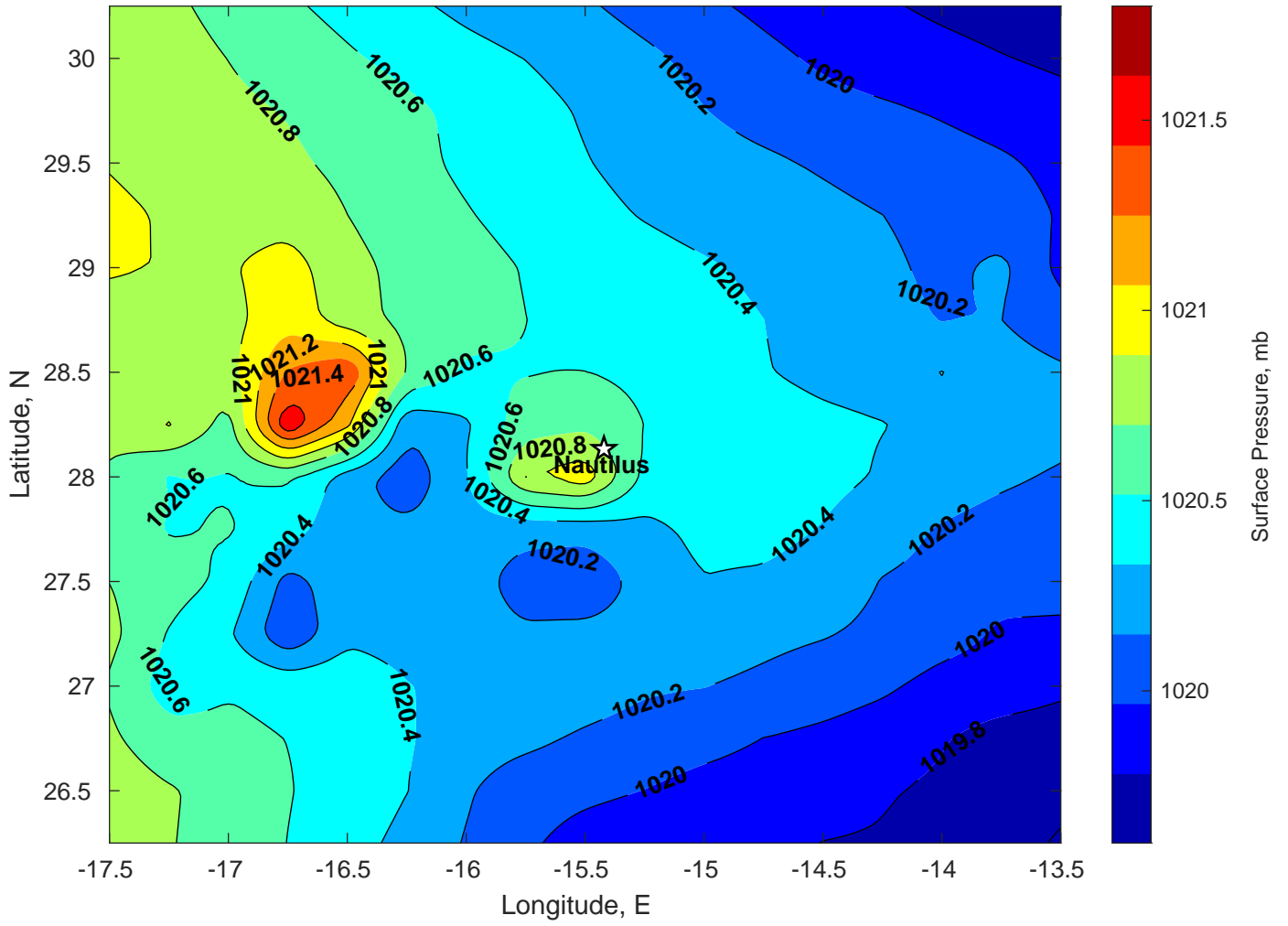
Surface Pressure (mb) for Nautilus at 21-Mar-2025 00:00:00
