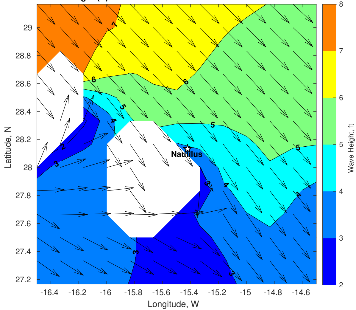
Wave Height (ft) for Nautilus at 19-Mar-2025 09:00:00
