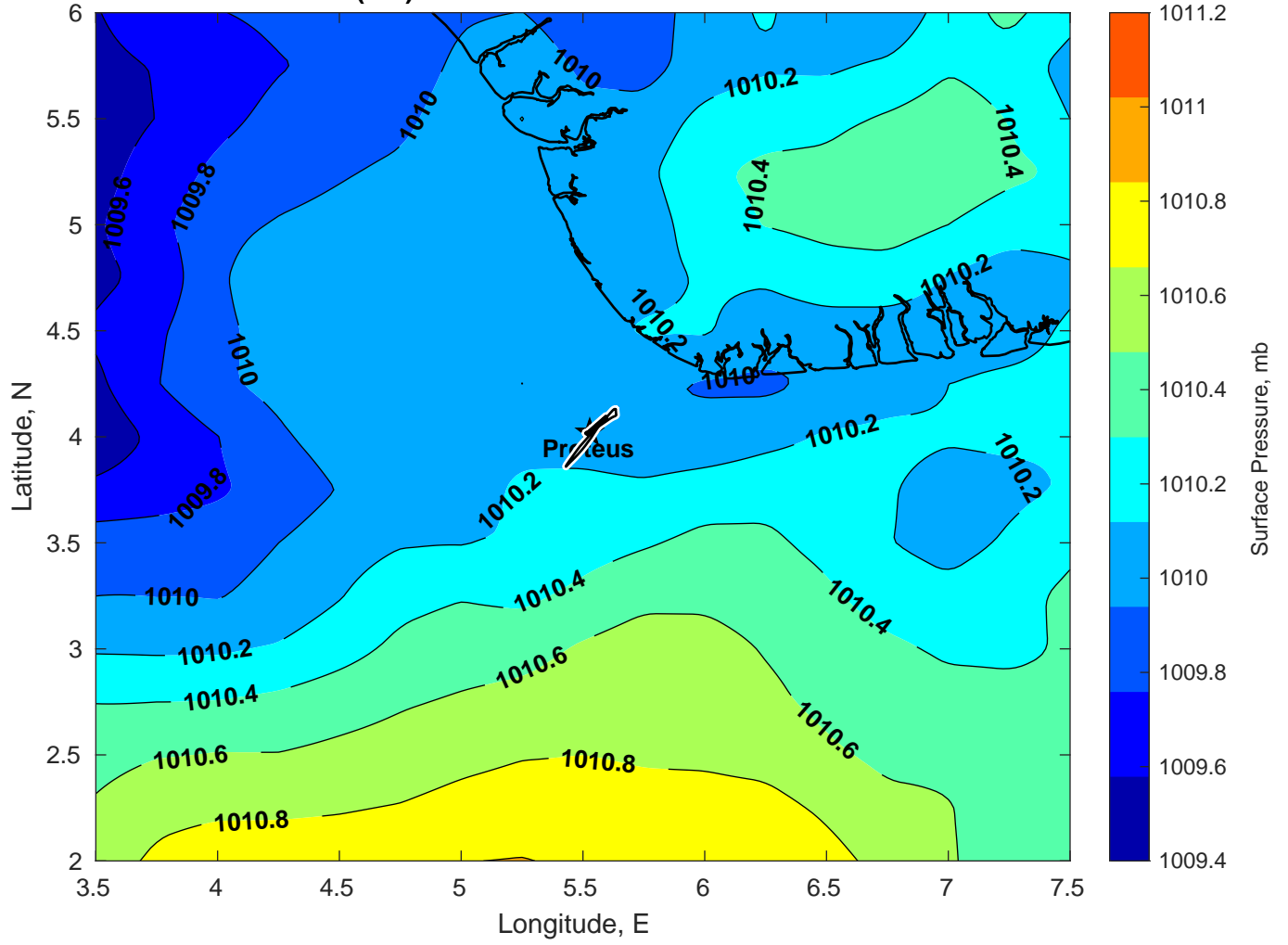
Surface Pressure (mb) for Proteus at 19-Mar-2025 00:00:00
