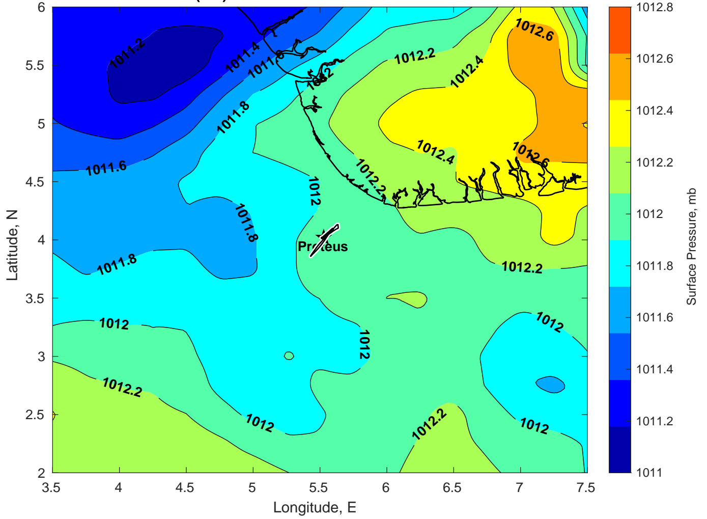
Surface Pressure (mb) for Proteus at 20-Mar-2025 00:00:00
