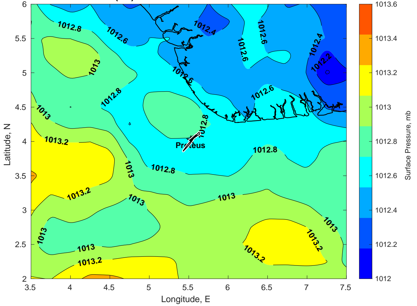
Surface Pressure (mb) for Proteus at 21-Mar-2025 00:00:00
