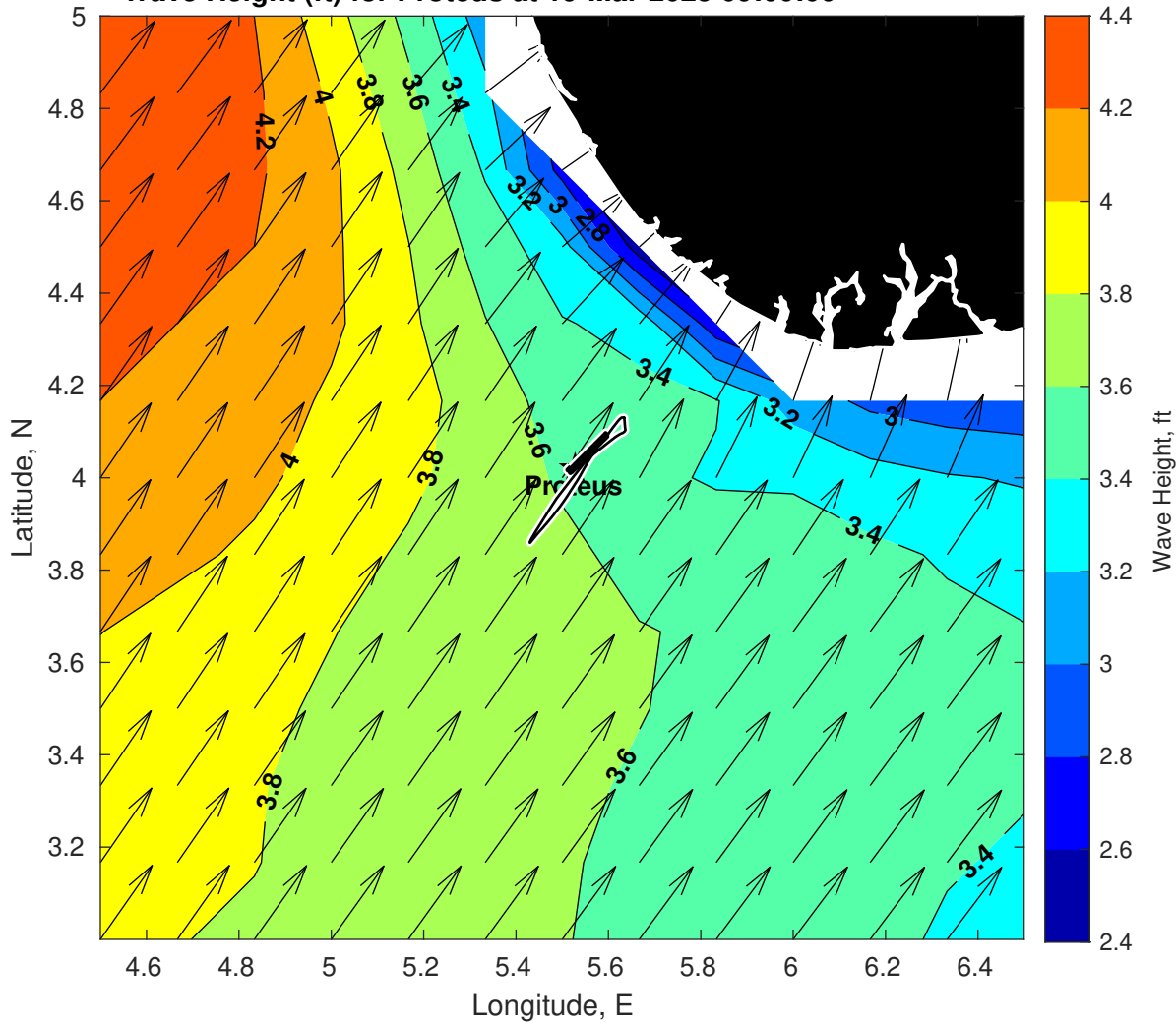
Wave Height (ft) for Proteus at 19-Mar-2025 09:00:00
