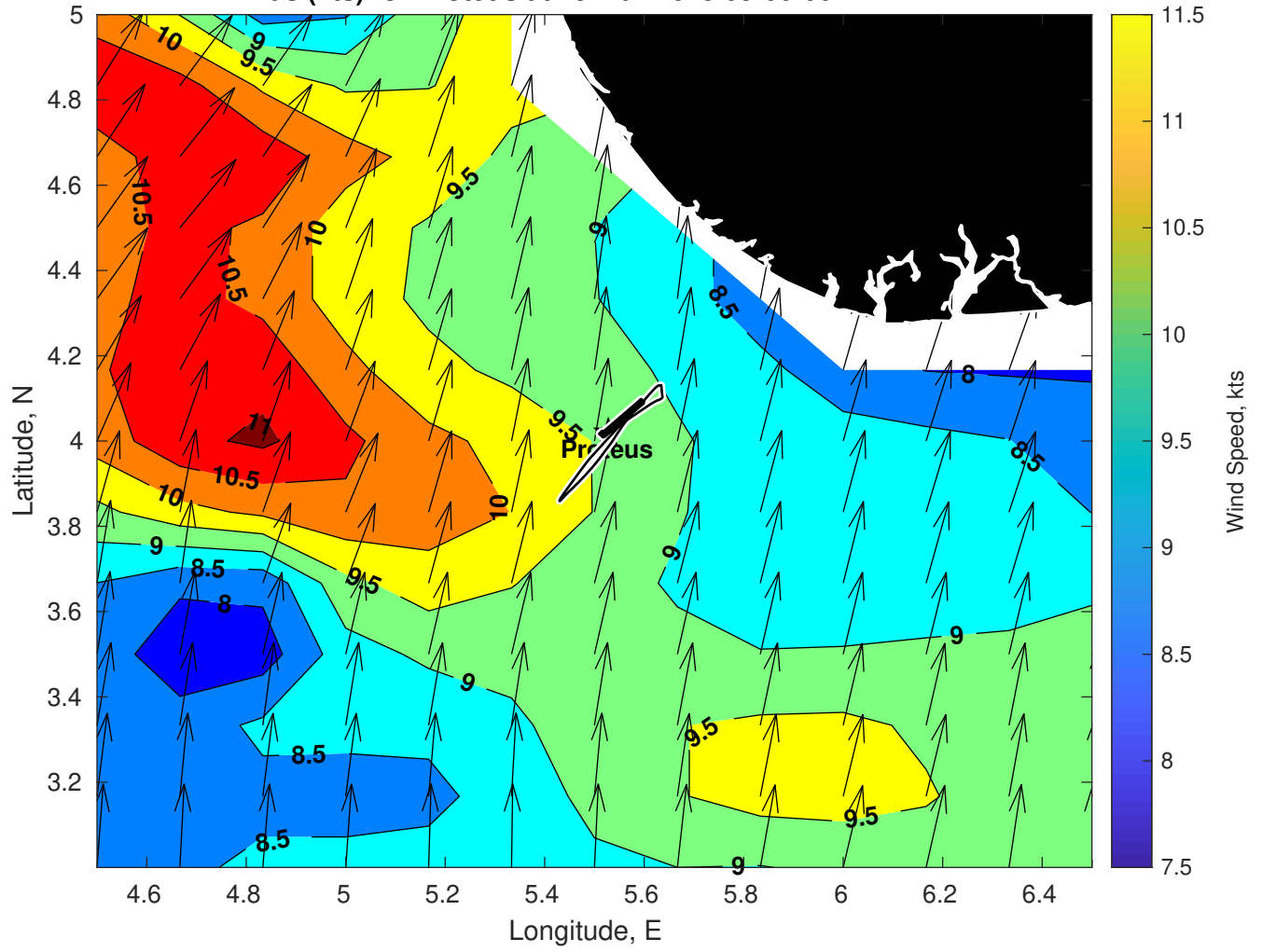
Winds (kts) for Proteus at 19-Mar-2025 09:00:00
