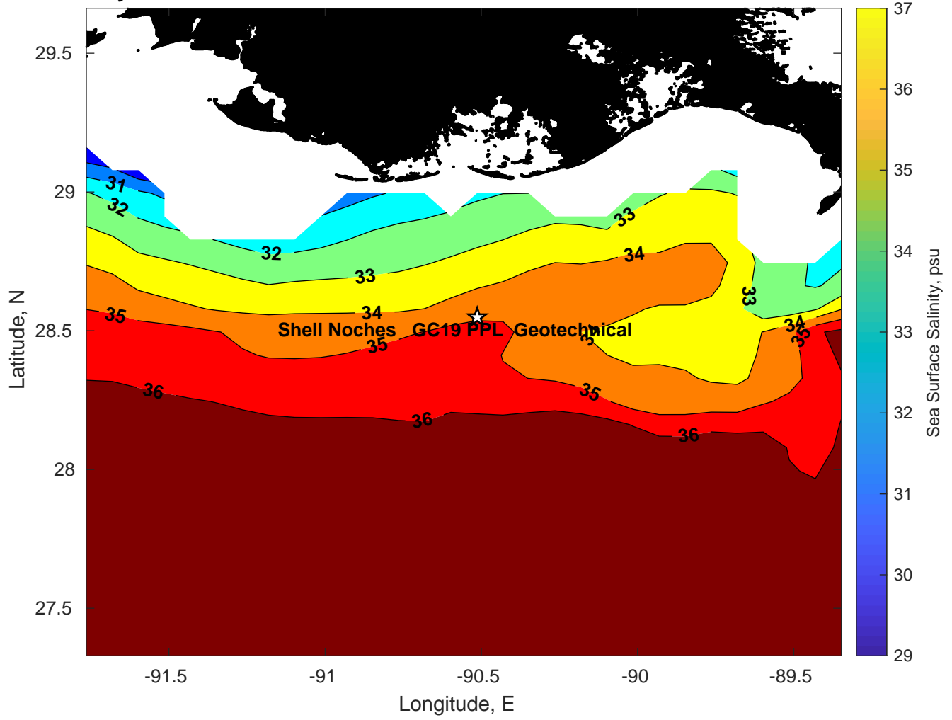
Surface Salinity for Shell Noches GC19 PPL Geotechnical at 18-Mar-2025 00:00:00
