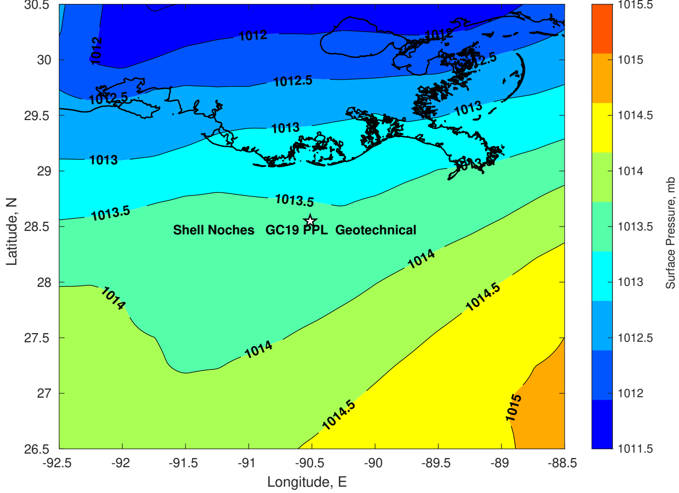
Surface Pressure (mb) for Shell Noches GC19 PPL Geotechnical at 20-Mar-2025 00:00:00
