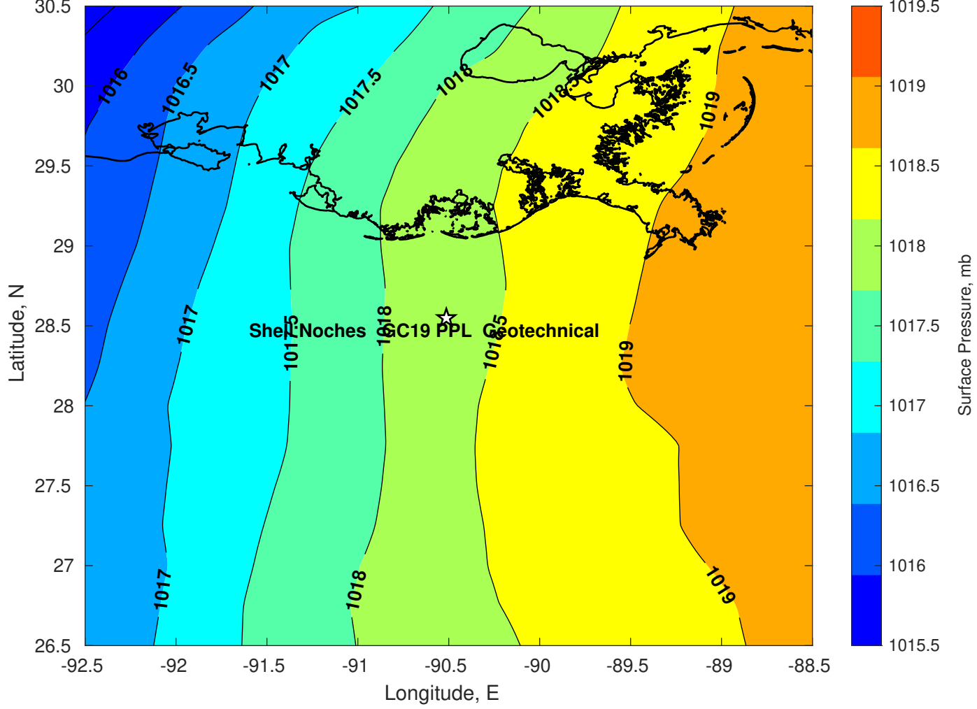
Surface Pressure (mb) for Shell Noches GC19 PPL Geotechnical at 19-Mar-2025 00:00:00
