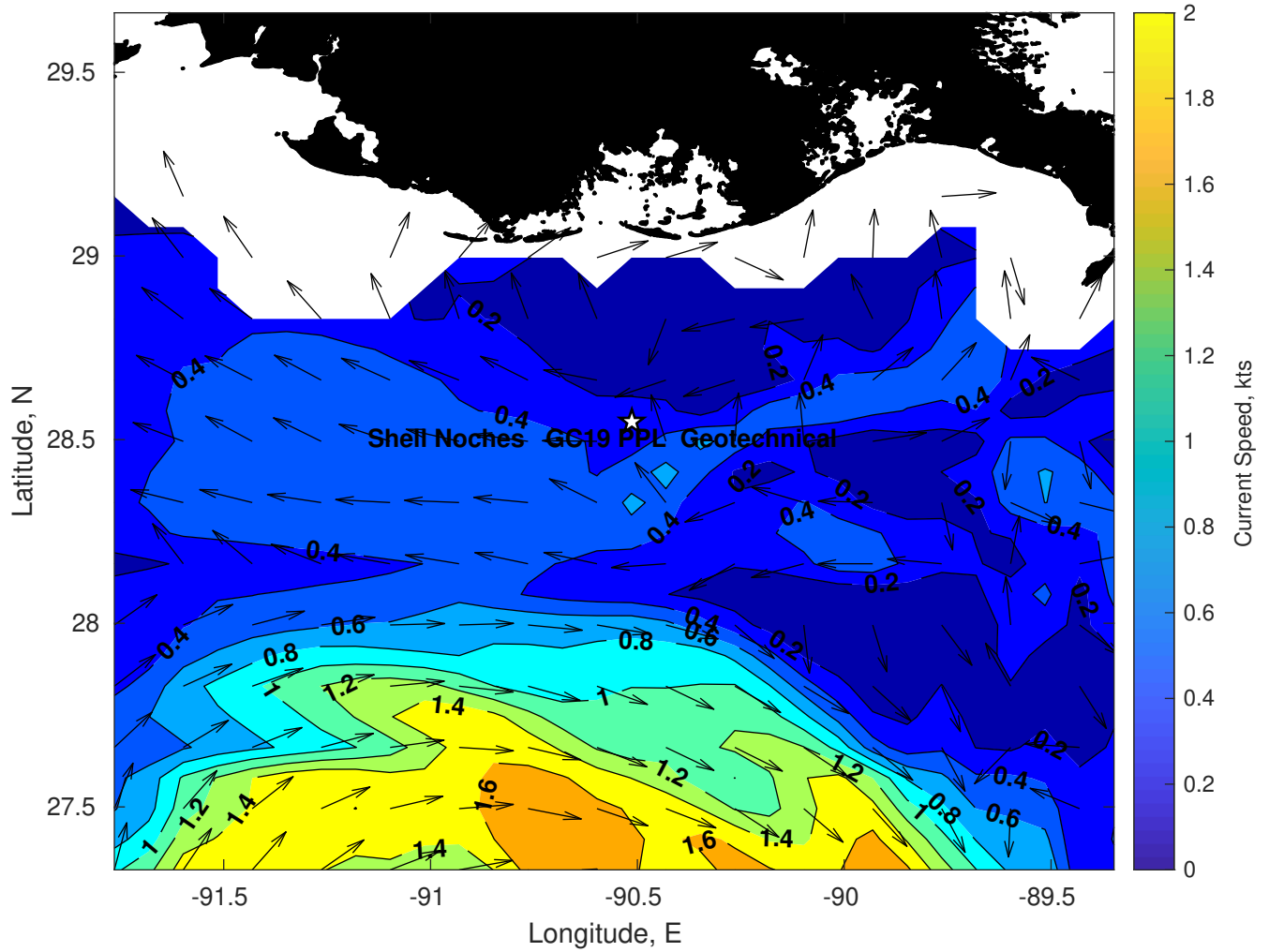
Surface Currents for Shell Noches GC19 PPL Geotechnical at 18-Mar-2025 00:00:00
