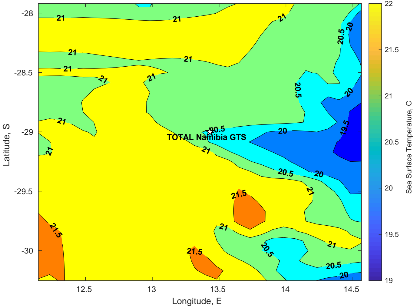
SST for TOTAL Namibia GTS at 18-Mar-2025 00:00:00
