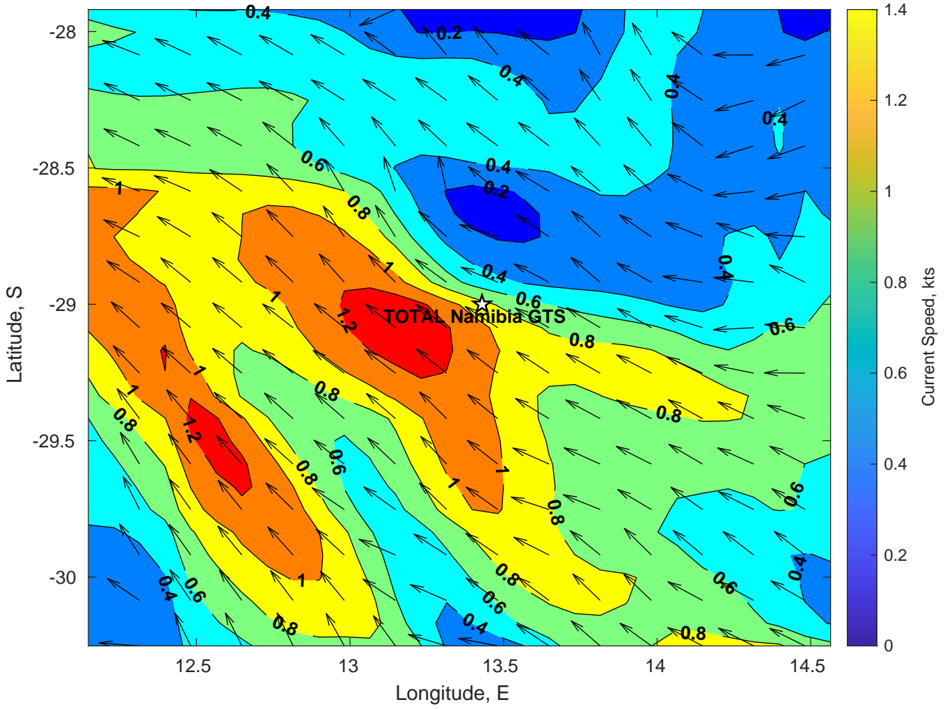
Surface Currents for TOTAL Namibia GTS at 18-Mar-2025 00:00:00
