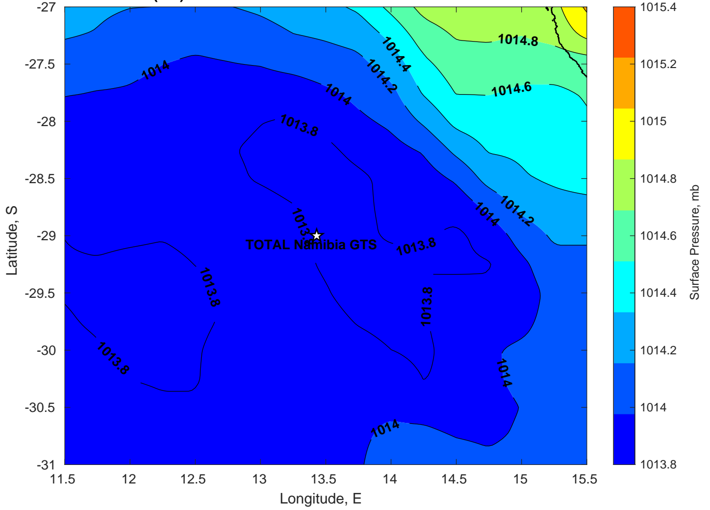
Surface Pressure (mb) for TOTAL Namibia GTS at 21-Mar-2025 00:00:00
