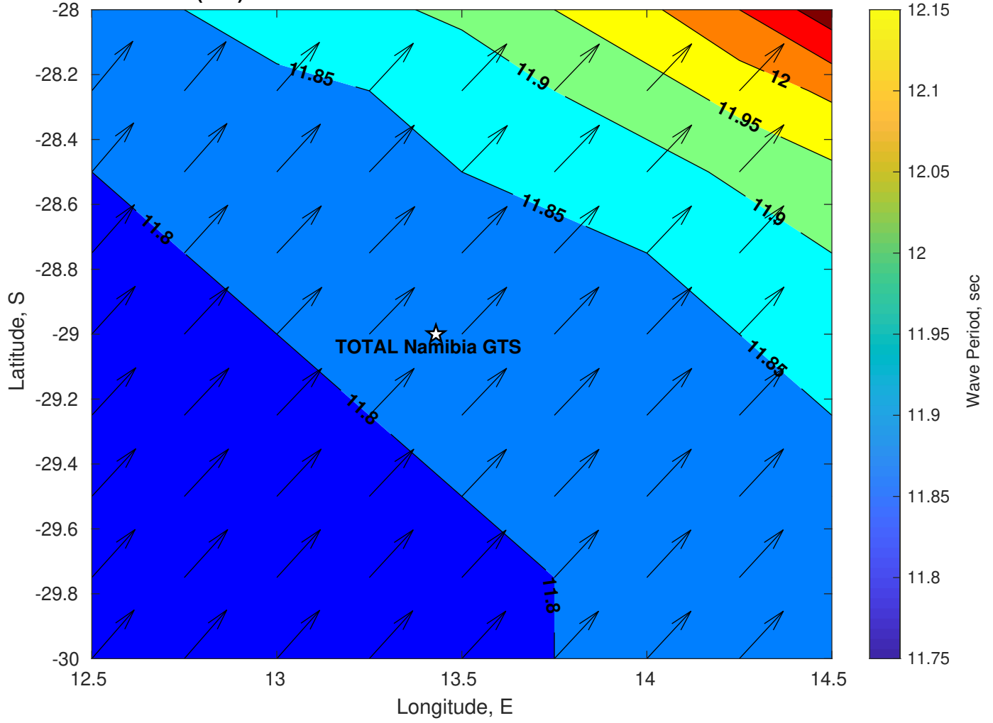
Wave Period (sec) for TOTAL Namibia GTS at 19-Mar-2025 09:00:00
