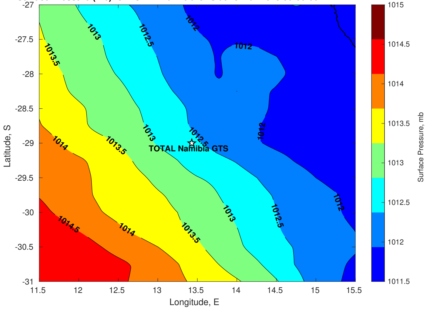
Surface Pressure (mb) for TOTAL Namibia GTS at 19-Mar-2025 00:00:00
