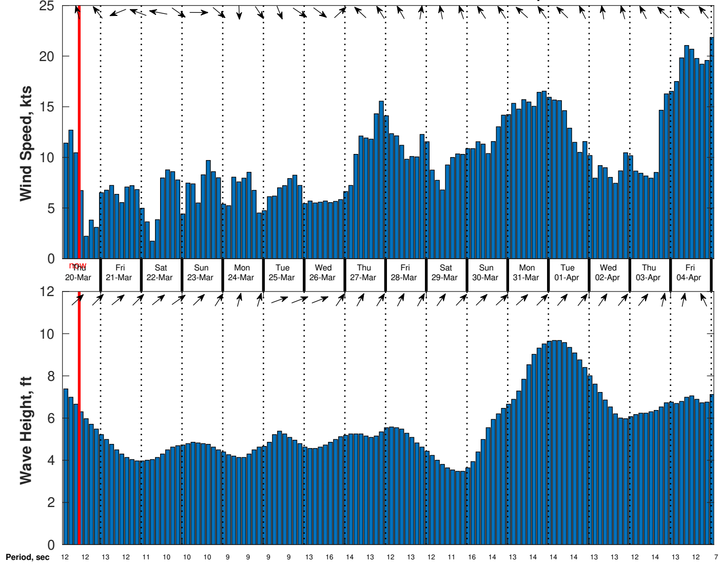
Wind & Wave Forecast for TOTAL Namibia GTS from 19-Mar-2025 02:00:00 to 04-Apr-2025 02:00:00
