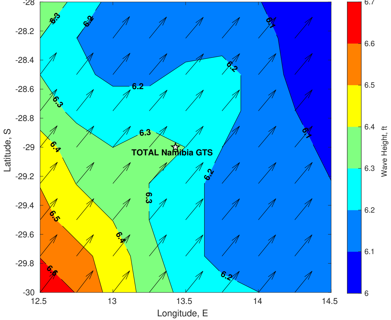
Wave Height (ft) for TOTAL Namibia GTS at 19-Mar-2025 09:00:00
