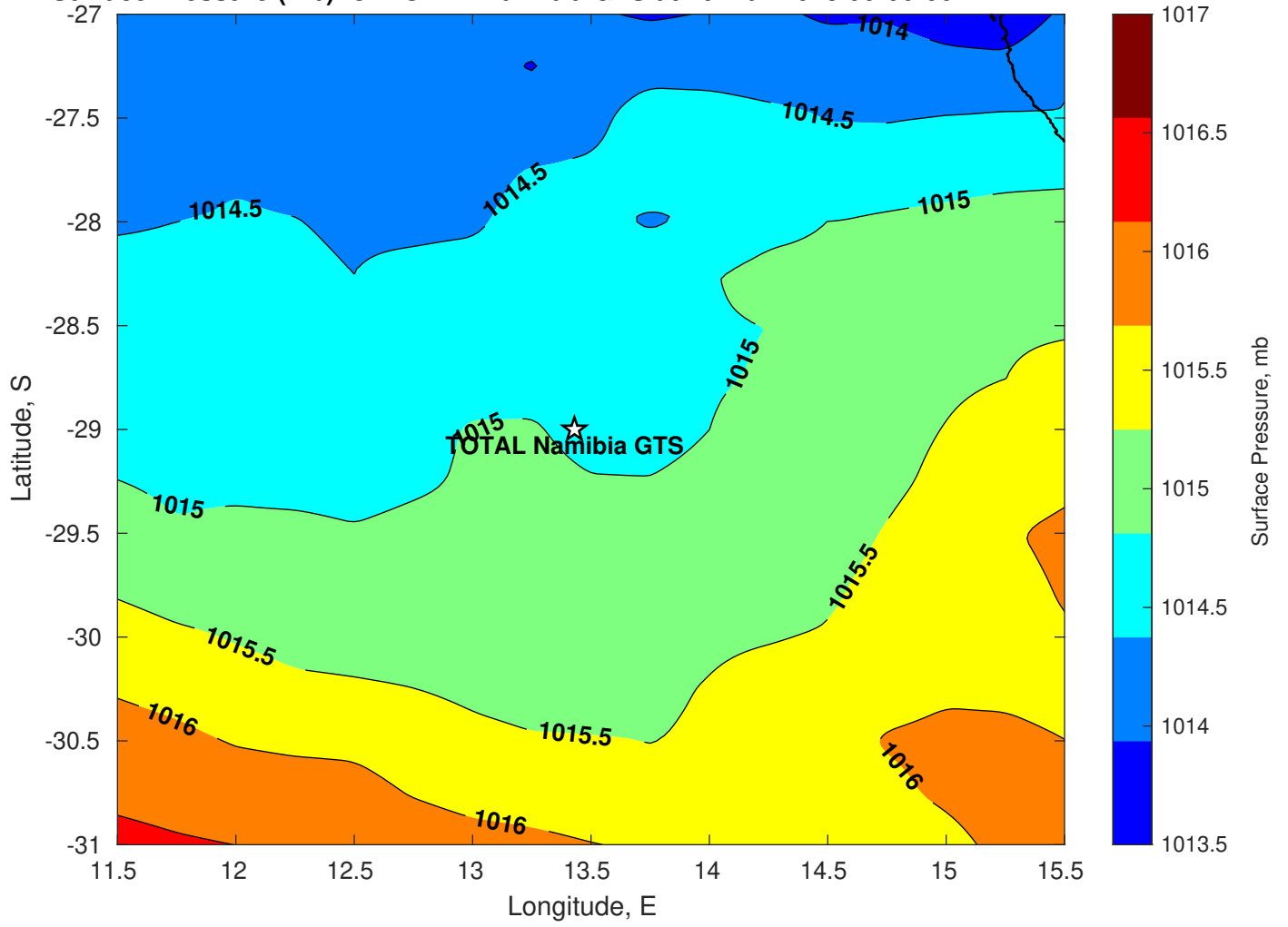
Surface Pressure (mb) for TOTAL Namibia GTS at 20-Mar-2025 00:00:00
