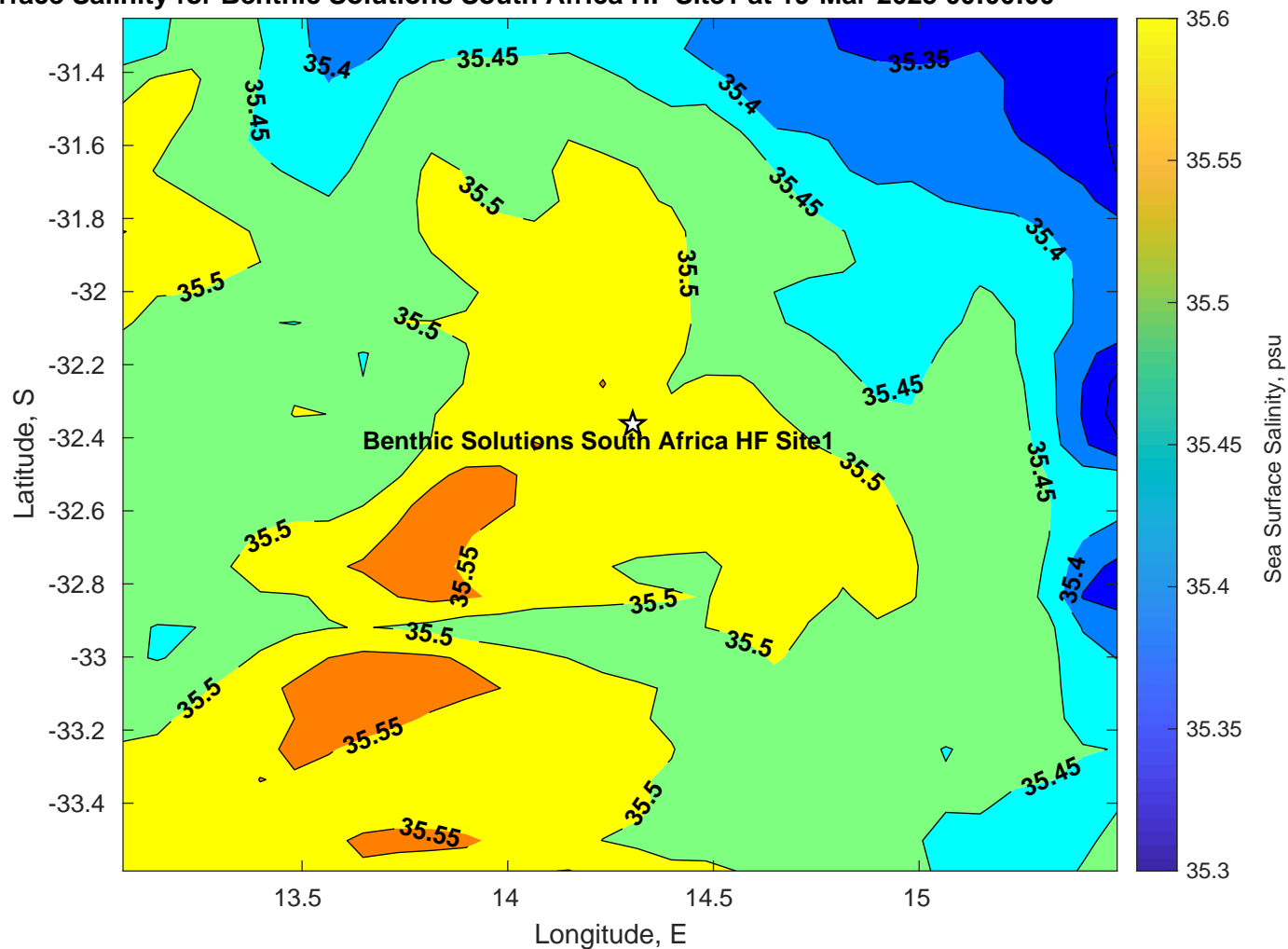
Surface Salinity for Benthic Solutions South Africa HF Site1 at 19-Mar-2025 00:00:00
