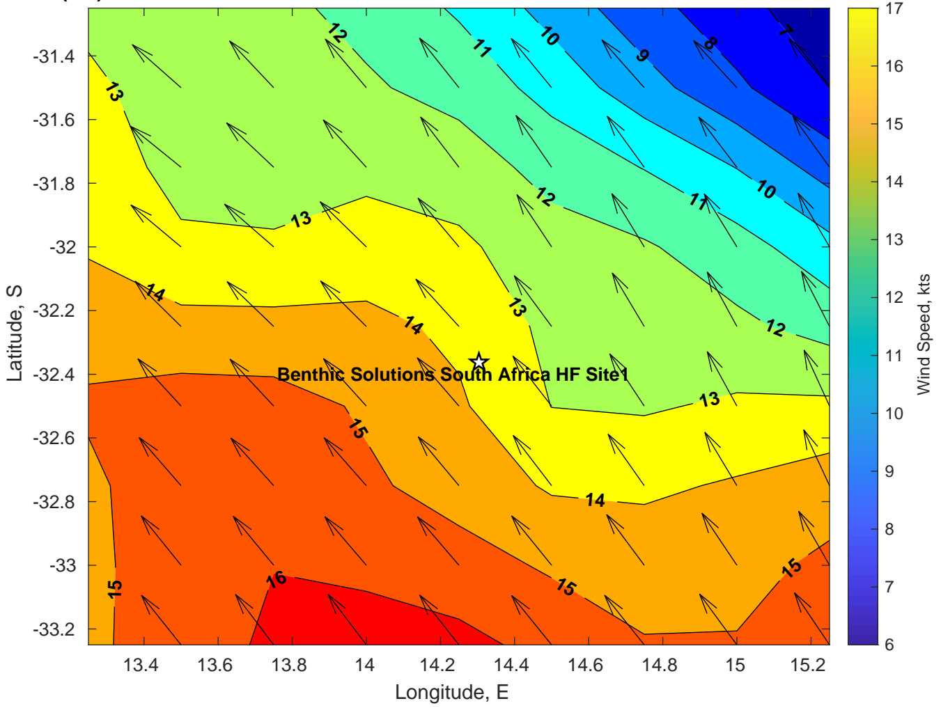
Winds (kts) for Benthic Solutions South Africa HF Site1 at 19-Mar-2025 21:00:00
