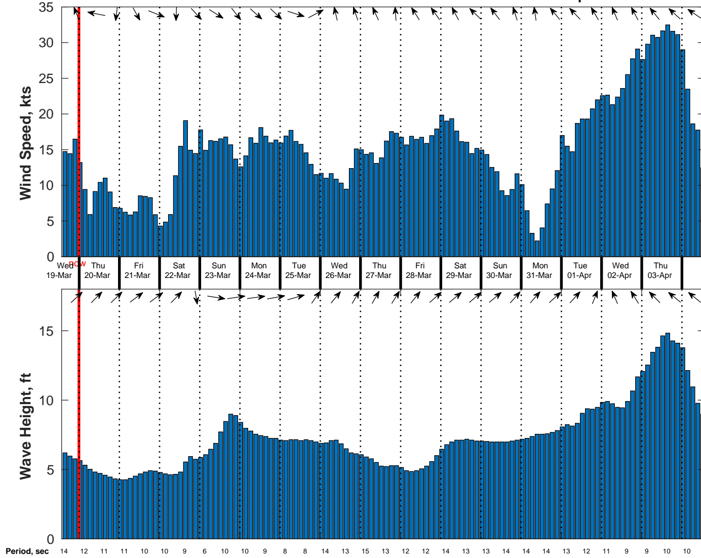
Wind & Wave Forecast for Benthic Solutions South Africa HF Site2 from 19-Mar-2025 14:00:00 to 04-Apr-2025 14:00:00
