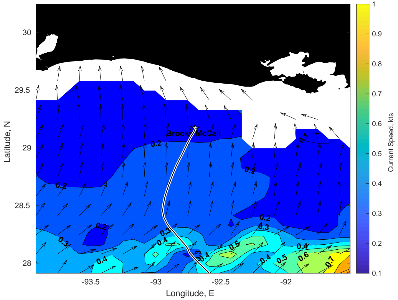
Surface Currents for Brooks McCall at 19-Mar-2025 00:00:00
