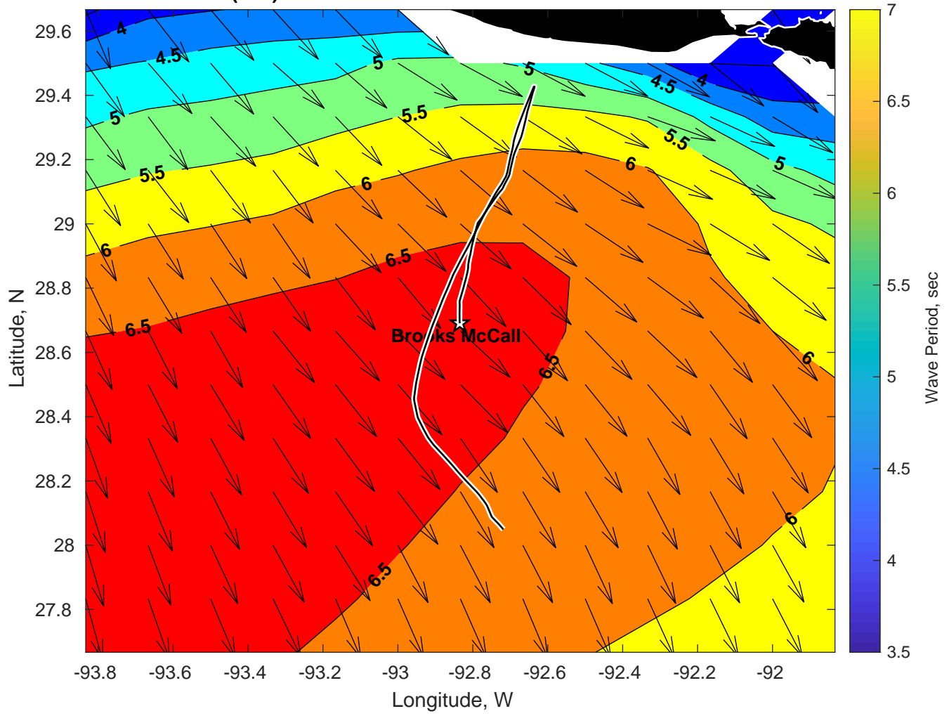
Wave Period (sec) for Brooks McCall at 20-Mar-2025 09:00:00
