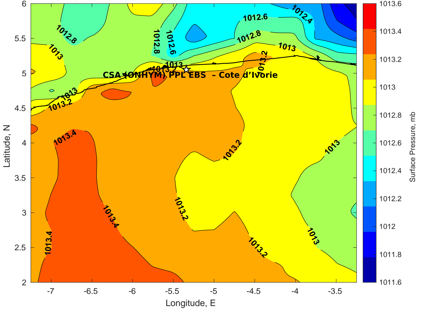
Surface Pressure (mb) for CSA (ONHYM) PPL EBS - Cote d'Ivoire at 20-Mar-2025 12:00:00
