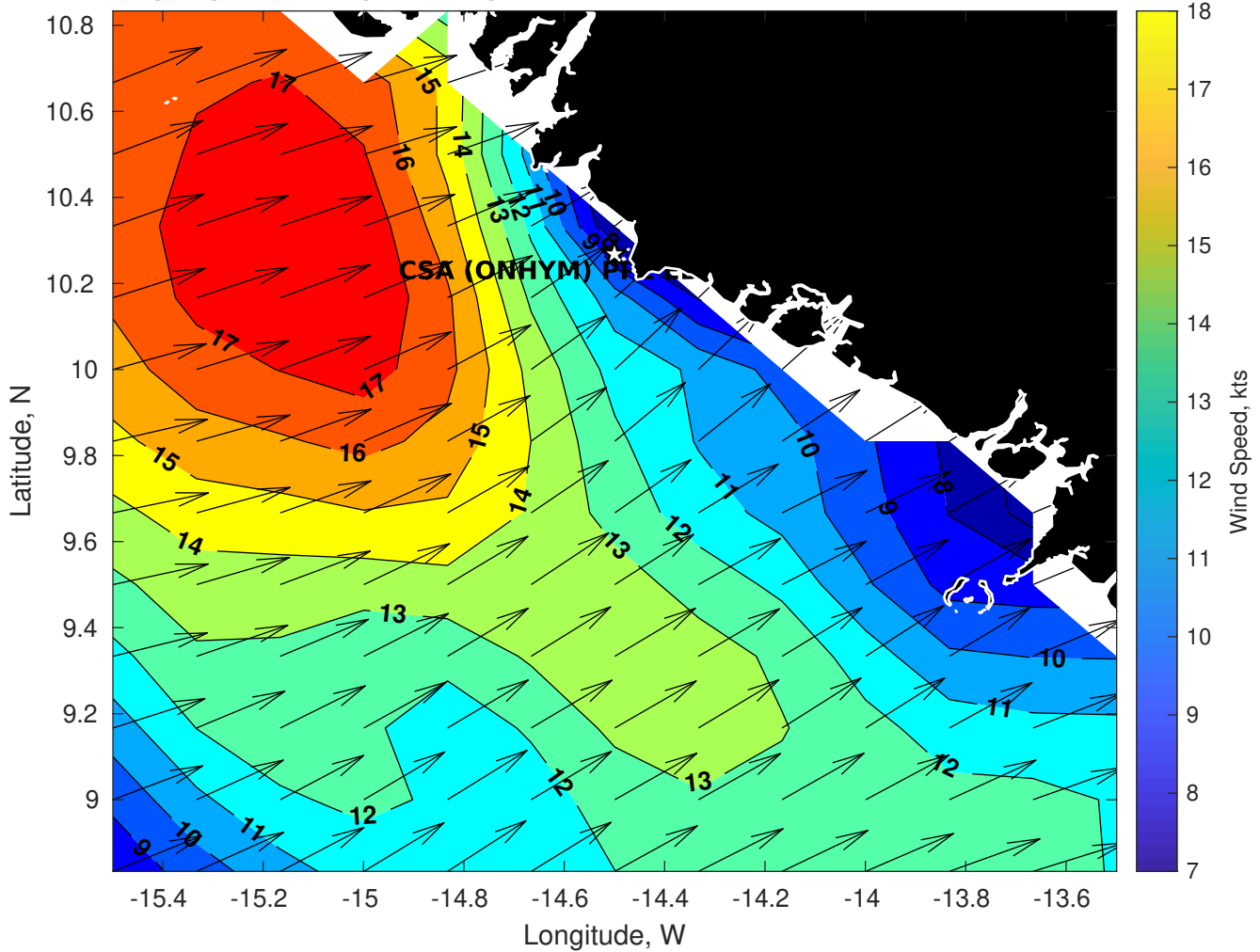
Winds (kts) for CSA (ONHYM) PPL EBS - Guinea at 19-Mar-2025 21:00:00
