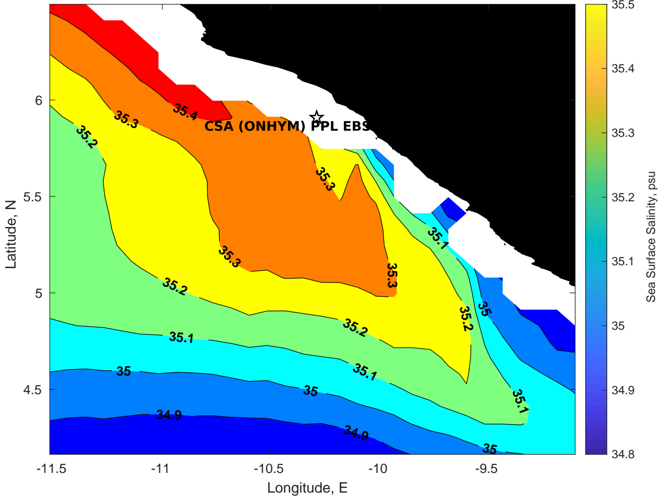
Surface Salinity for CSA (ONHYM) PPL EBS - Liberia at 19-Mar-2025 00:00:00
