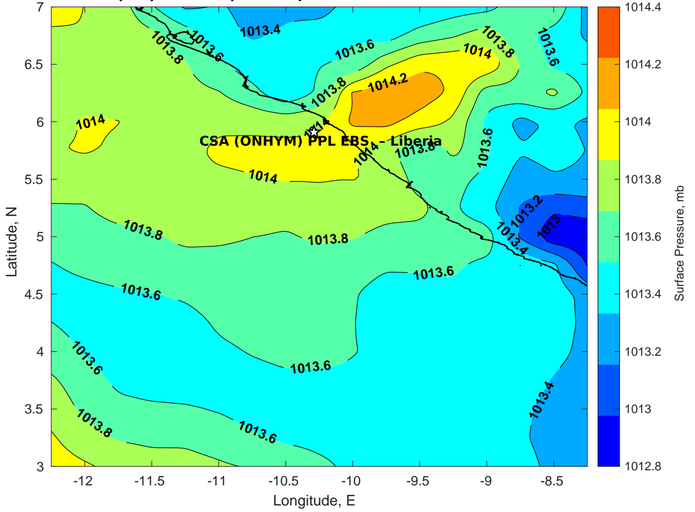
Surface Pressure (mb) for CSA (ONHYM) PPL EBS - Liberia at 20-Mar-2025 12:00:00
