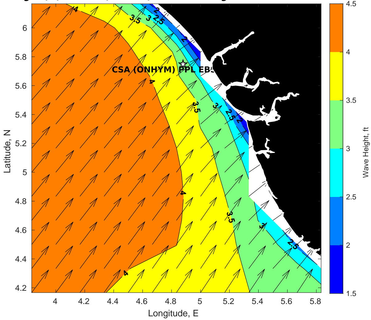
Wave Height (ft) for CSA (ONHYM) PPL EBS - Nigeria at 19-Mar-2025 21:00:00
