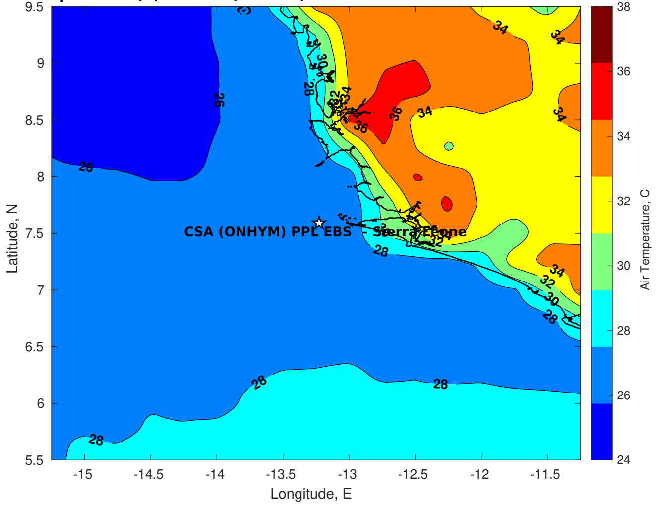
Air Temperature (C) for CSA (ONHYM) PPL EBS - Sierra Leone at 19-Mar-2025
