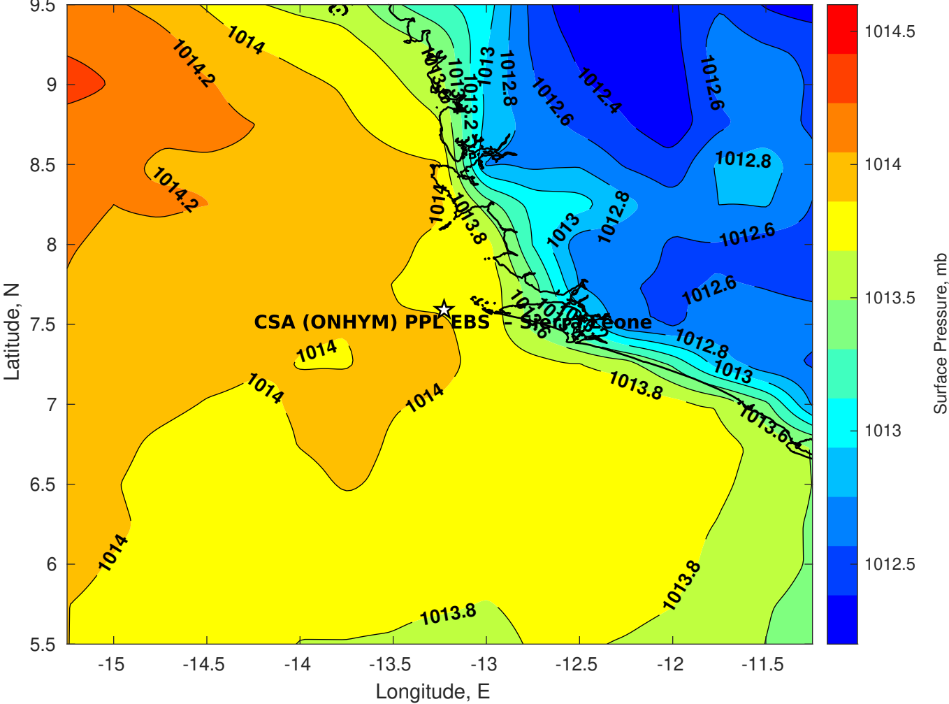
Surface Pressure (mb) for CSA (ONHYM) PPL EBS - Sierra Leone at 21-Mar-2025 12:00:00
