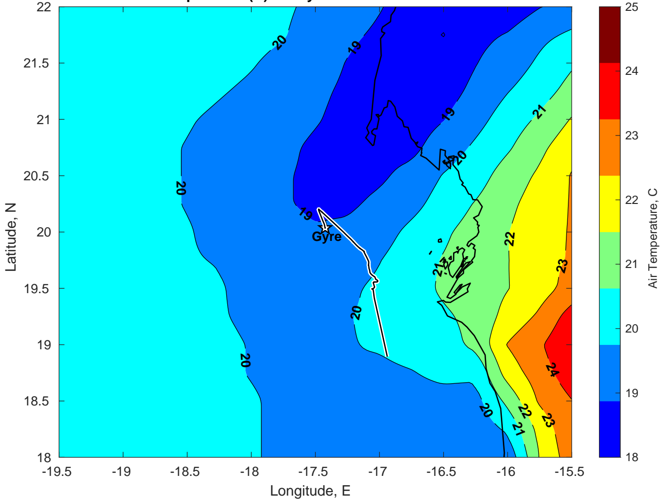
Air Temperature (C) for Gyre at 20-Mar-2025
