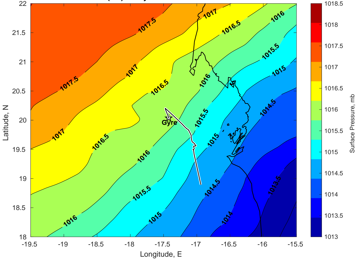
Surface Pressure (mb) for Gyre at 20-Mar-2025 00:00:00
