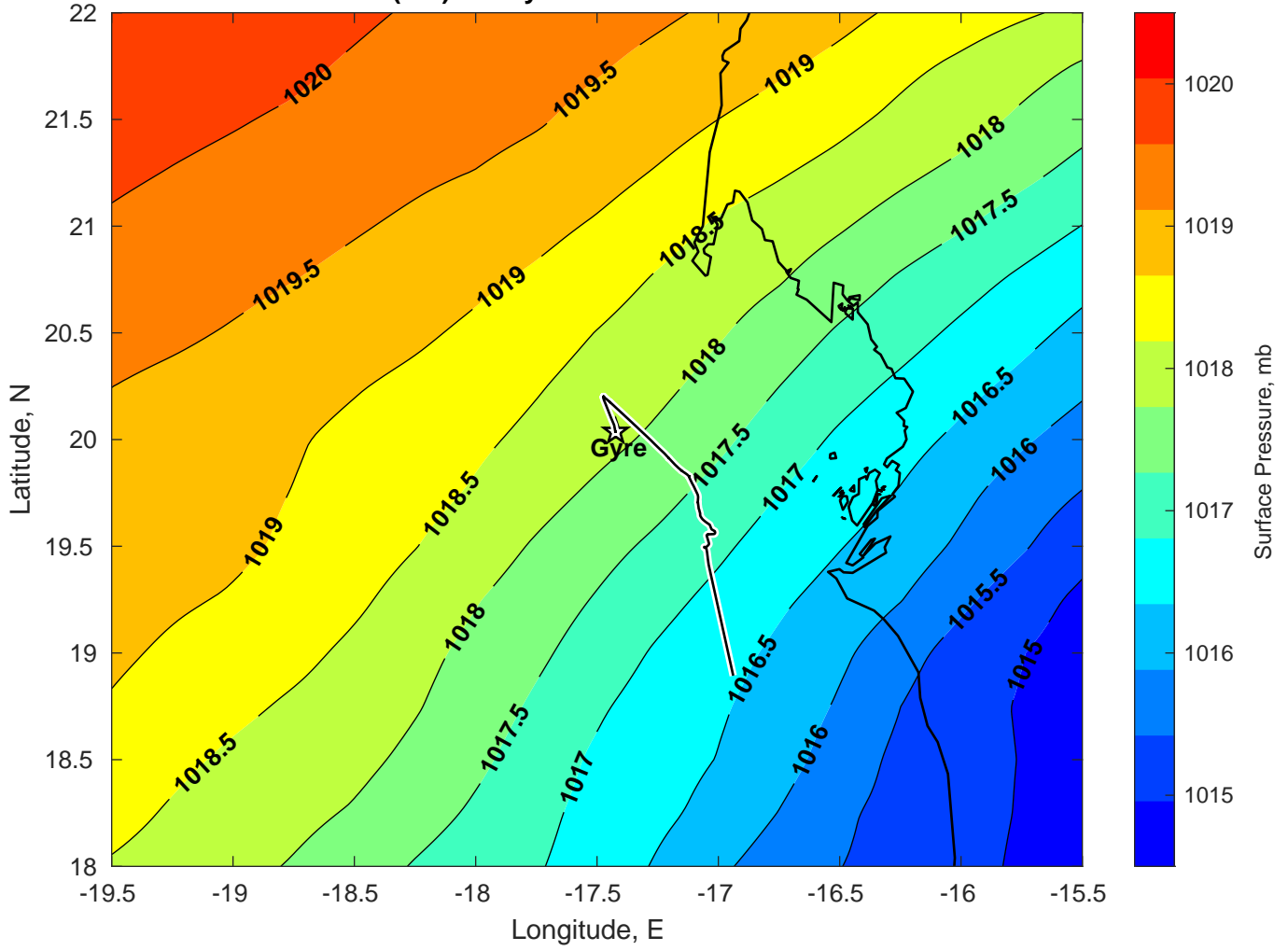
Surface Pressure (mb) for Gyre at 21-Mar-2025 00:00:00
