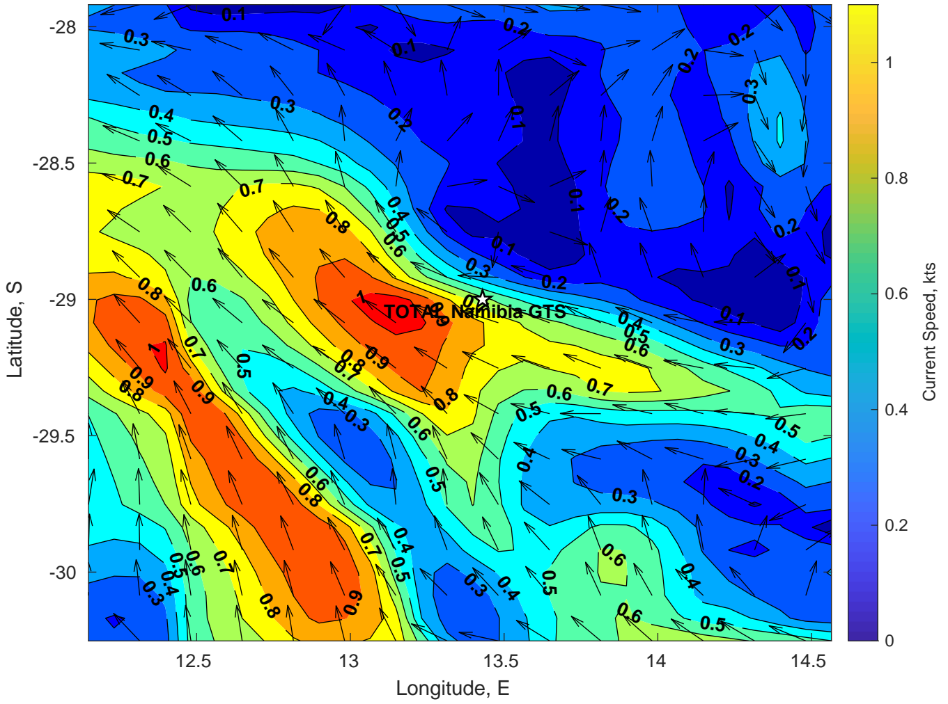
Surface Currents for TOTAL Namibia GTS at 19-Mar-2025 00:00:00
