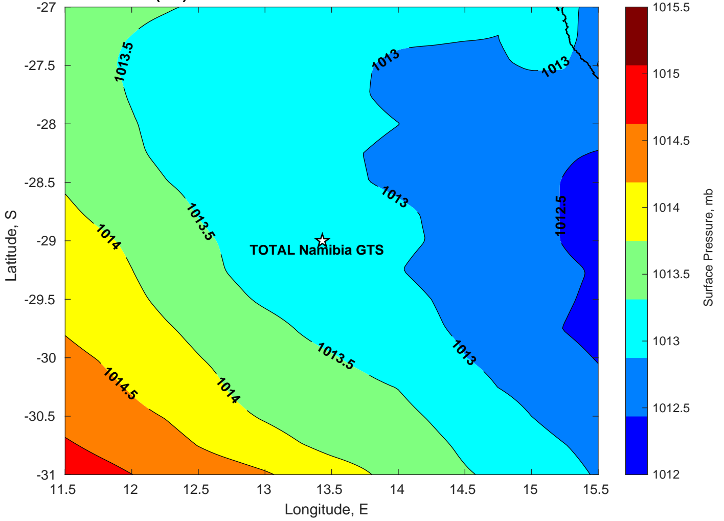
Surface Pressure (mb) for TOTAL Namibia GTS at 19-Mar-2025 12:00:00
