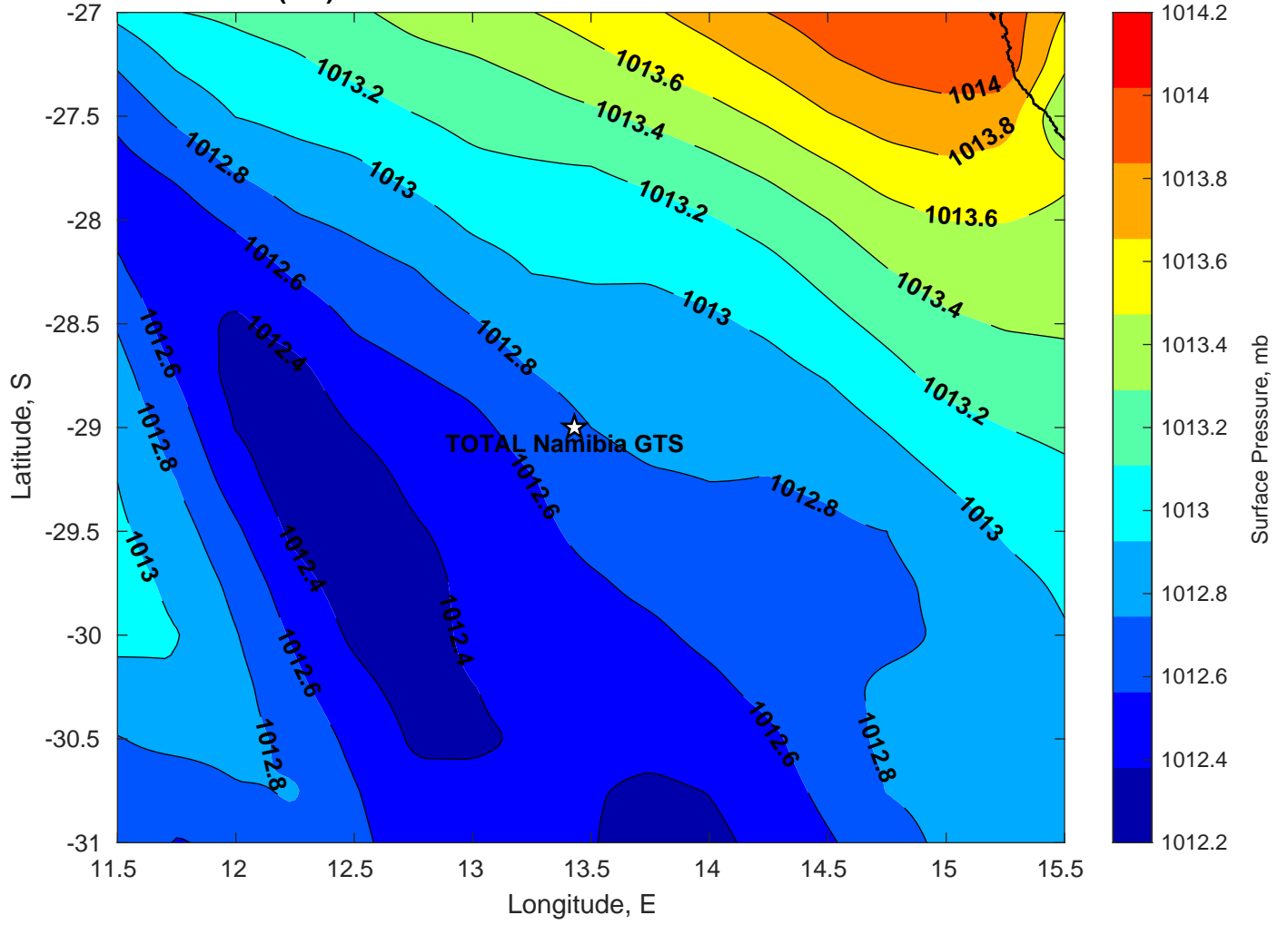
Surface Pressure (mb) for TOTAL Namibia GTS at 21-Mar-2025 12:00:00
