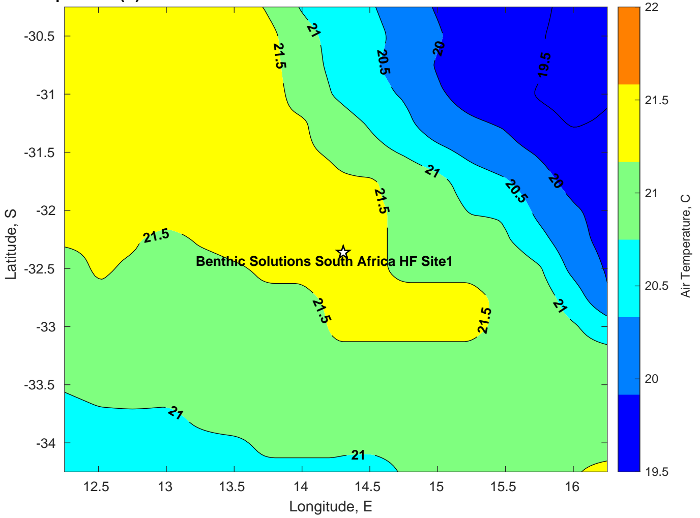
Air Temperature (C) for Benthic Solutions South Africa HF Site1 at 19-Mar-2025
