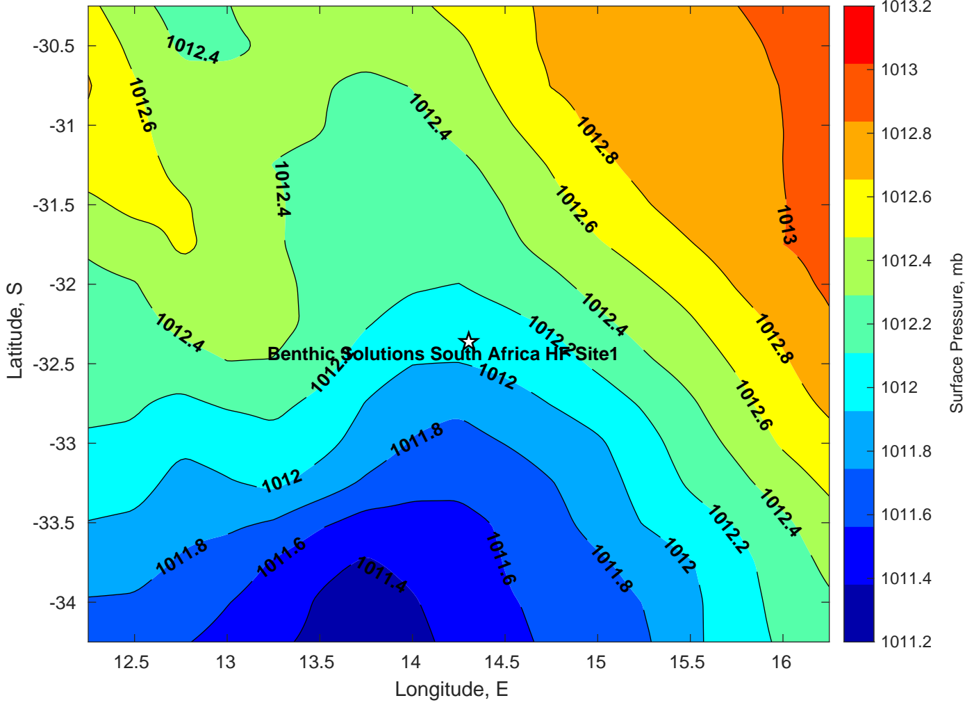
Surface Pressure (mb) for Benthic Solutions South Africa HF Site1 at 21-Mar-2025 12:00:00
