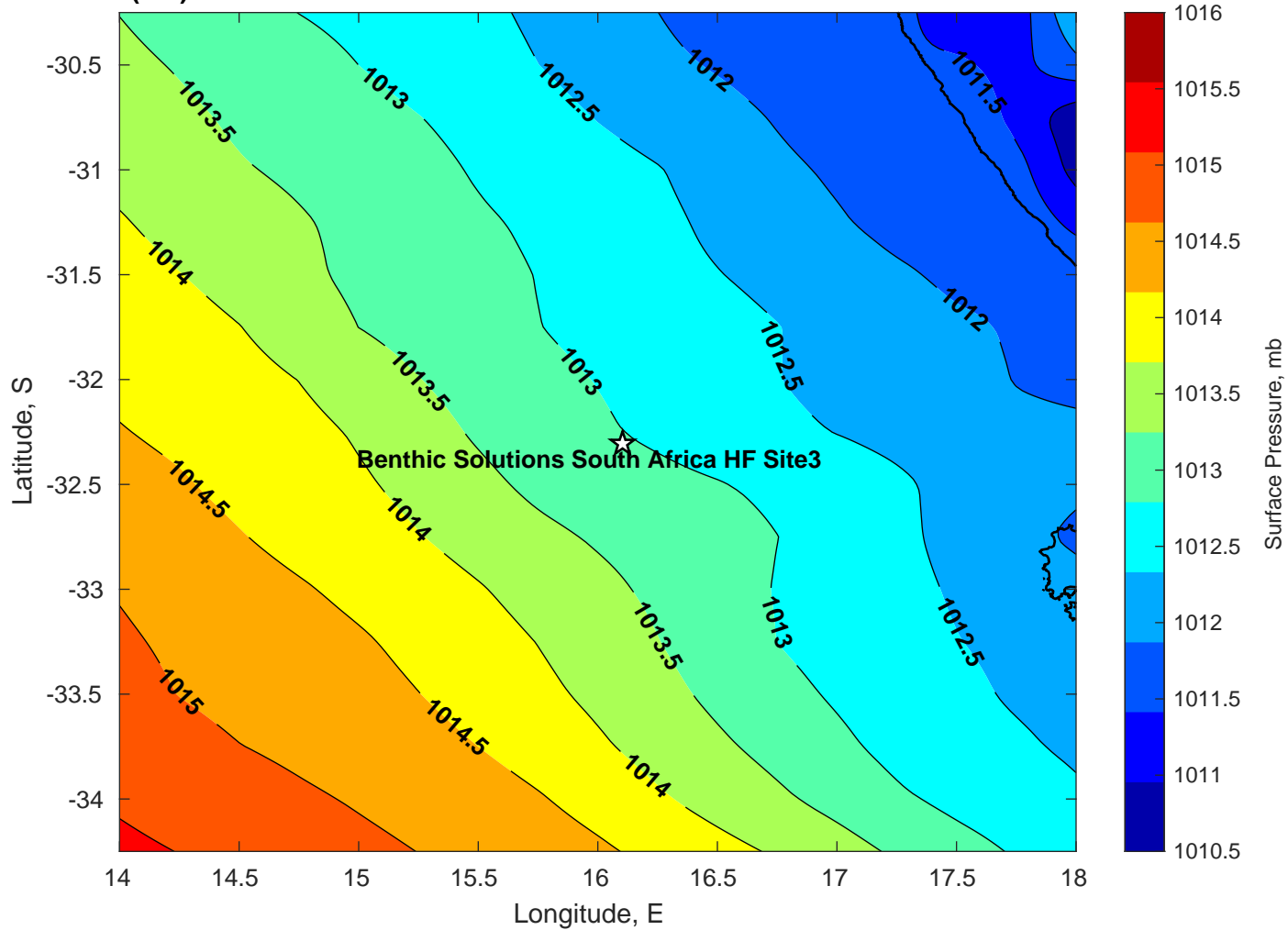
Surface Pressure (mb) for Benthic Solutions South Africa HF Site3 at 19-Mar-2025 12:00:00
