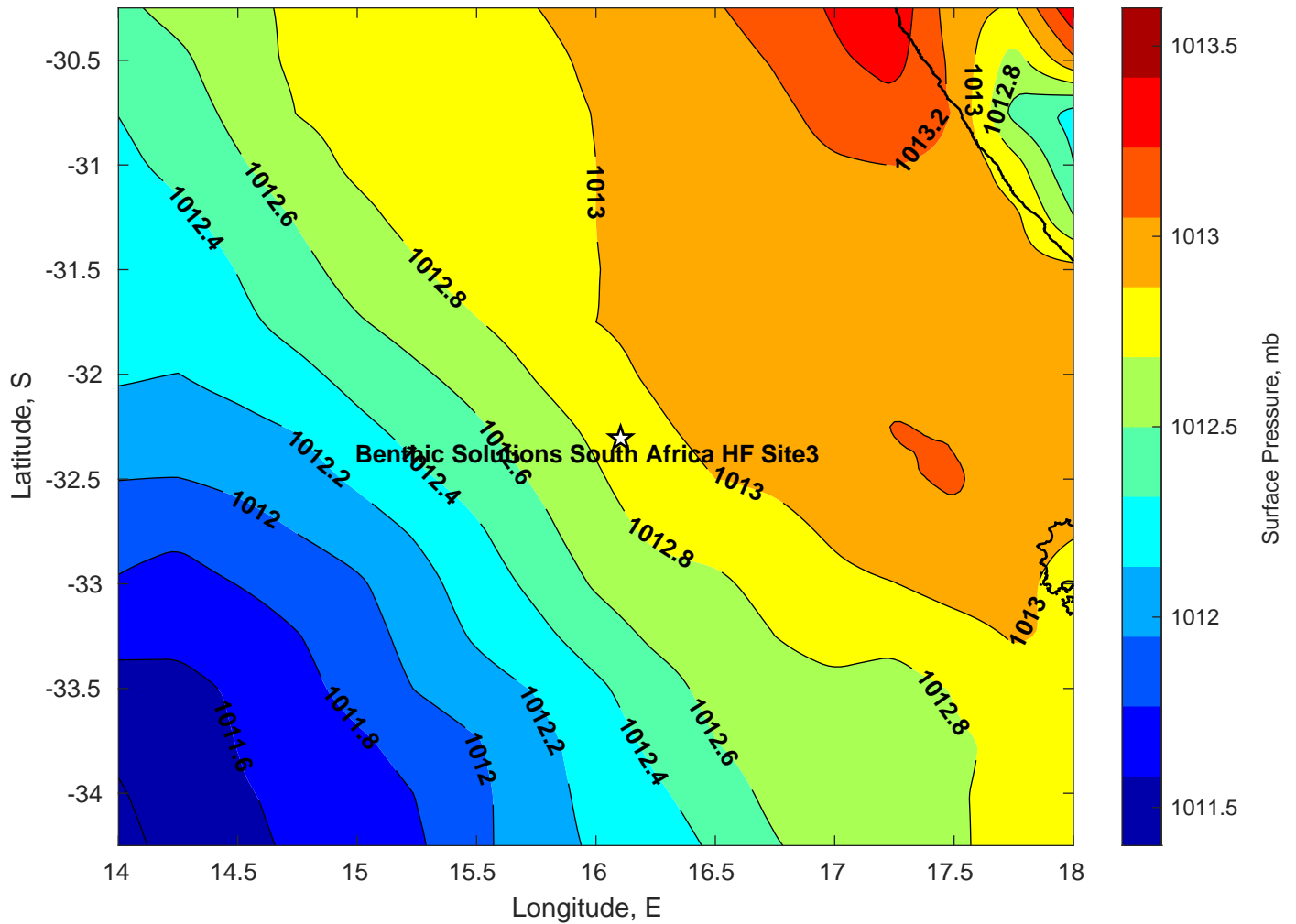
Surface Pressure (mb) for Benthic Solutions South Africa HF Site3 at 21-Mar-2025 12:00:00
