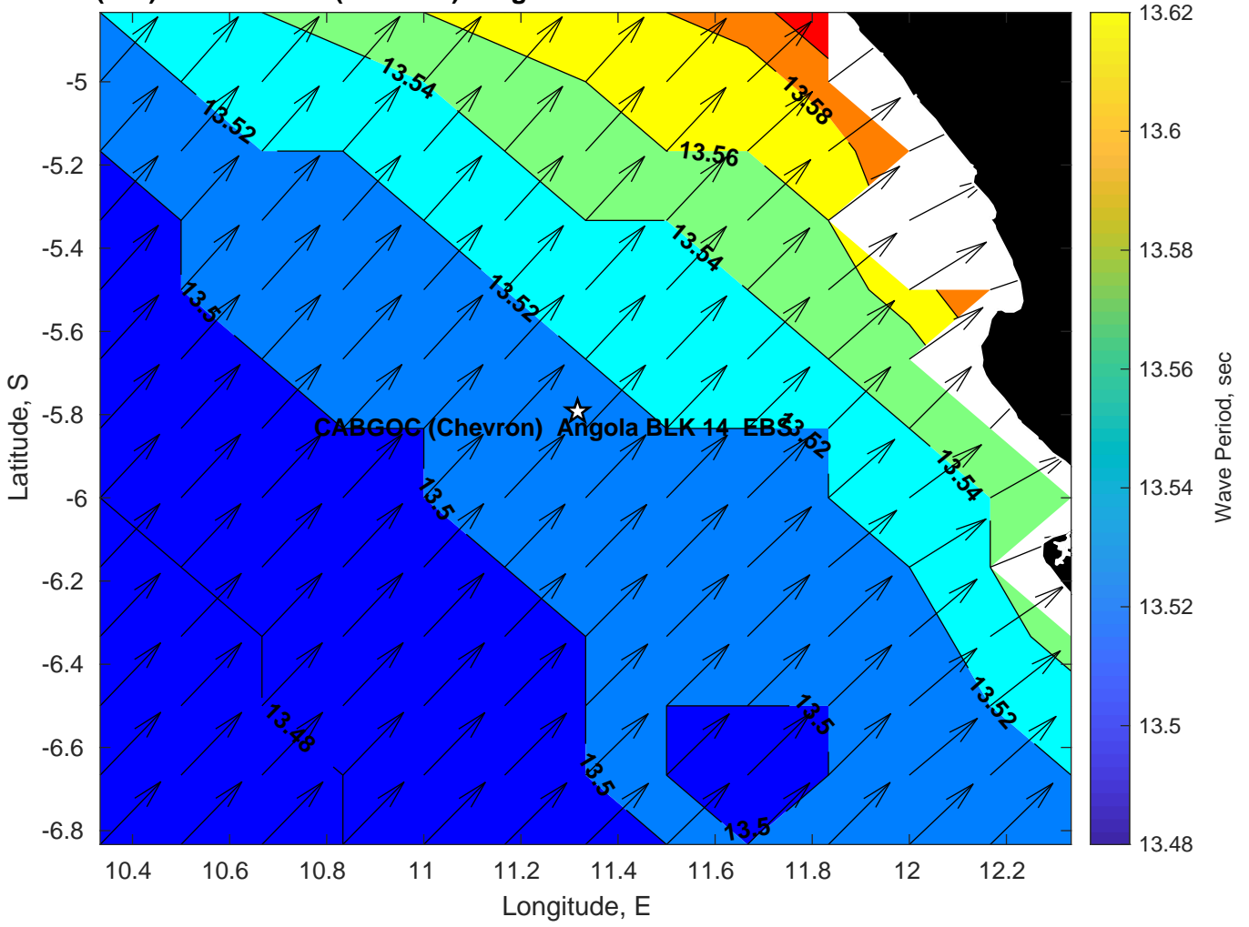
Wave Period (sec) for CABGOC (Chevron) Angola BLK 14 EBS at 19-Mar-2025 21:00:00
