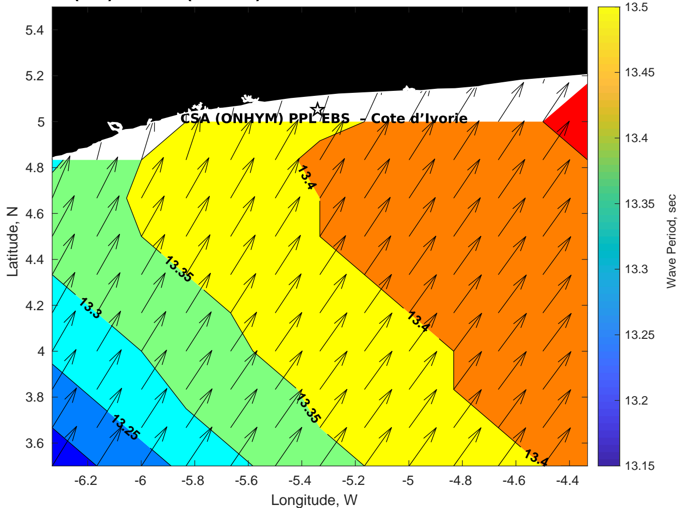
Wave Period (sec) for CSA (ONHYM) PPL EBS - Cote d'Ivoire at 19-Mar-2025 21:00:00
