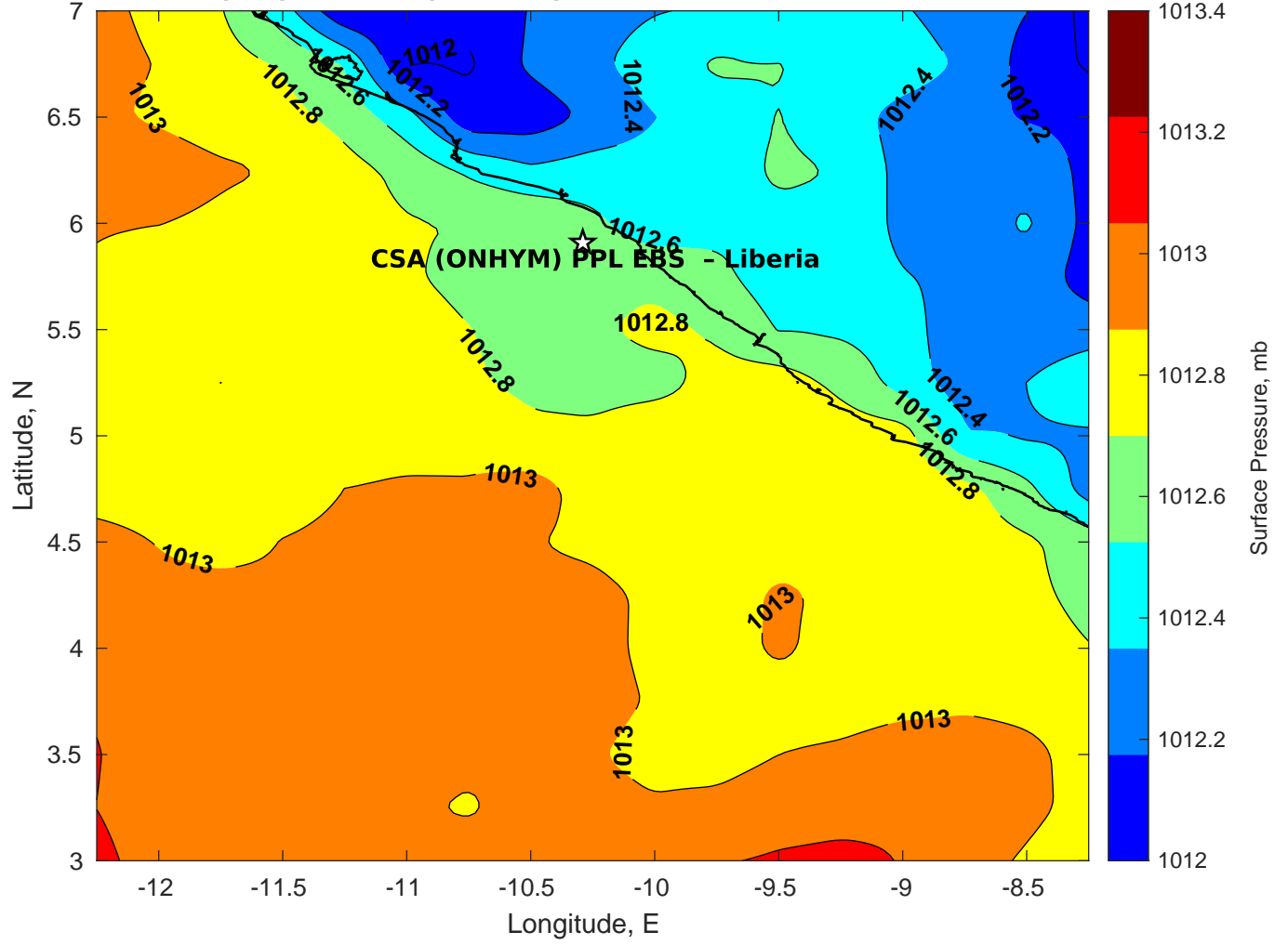
Surface Pressure (mb) for CSA (ONHYM) PPL EBS - Liberia at 19-Mar-2025 12:00:00
