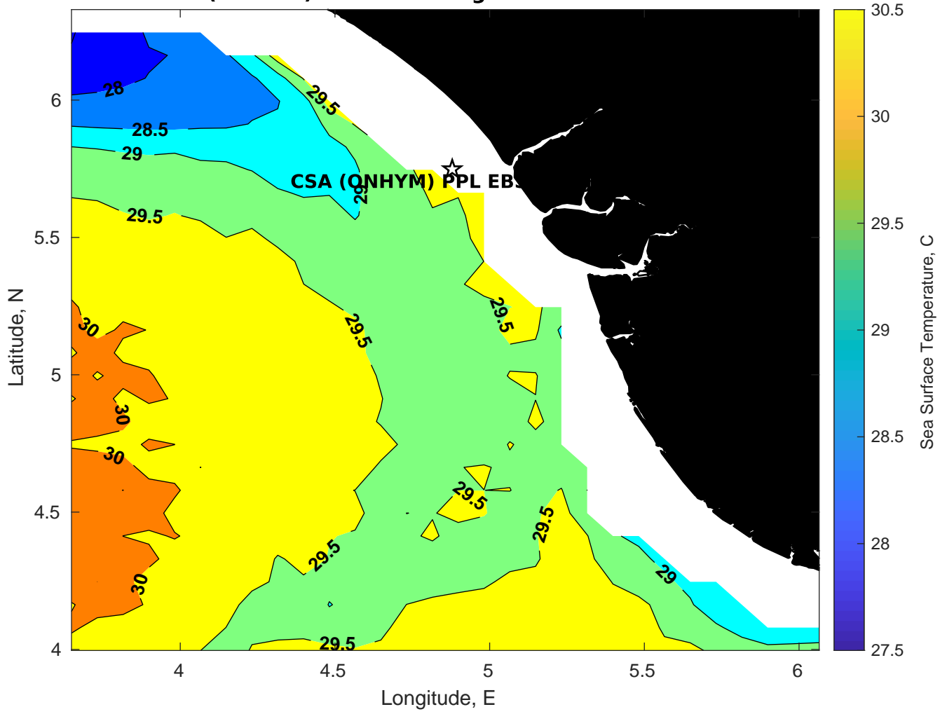
SST for CSA (ONHYM) PPL EBS - Nigeria at 19-Mar-2025 00:00:00
