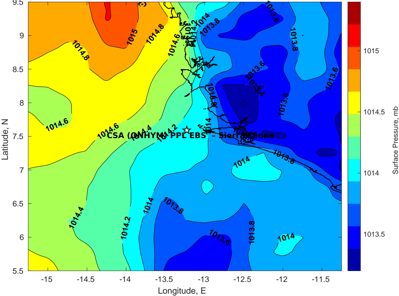
Surface Pressure (mb) for CSA (ONHYM) PPL EBS - Sierra Leone at 20-Mar-2025 12:00:00
