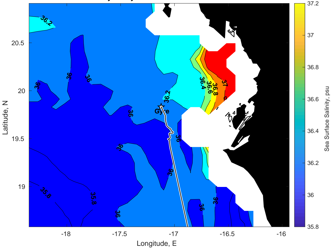
Surface Salinity for Gyre at 19-Mar-2025 00:00:00
