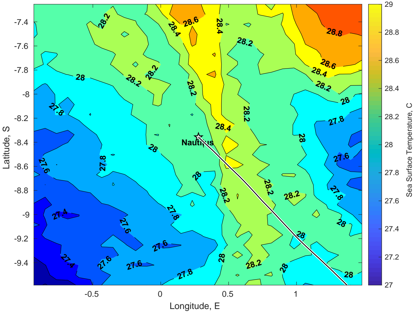
SST for Nautilus at 19-Mar-2025 00:00:00
