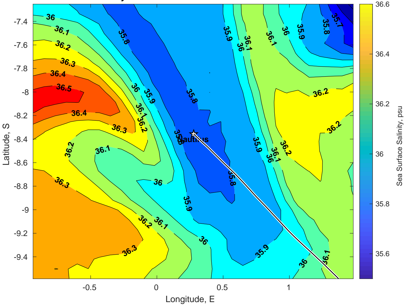
Surface Salinity for Nautilus at 19-Mar-2025 00:00:00
