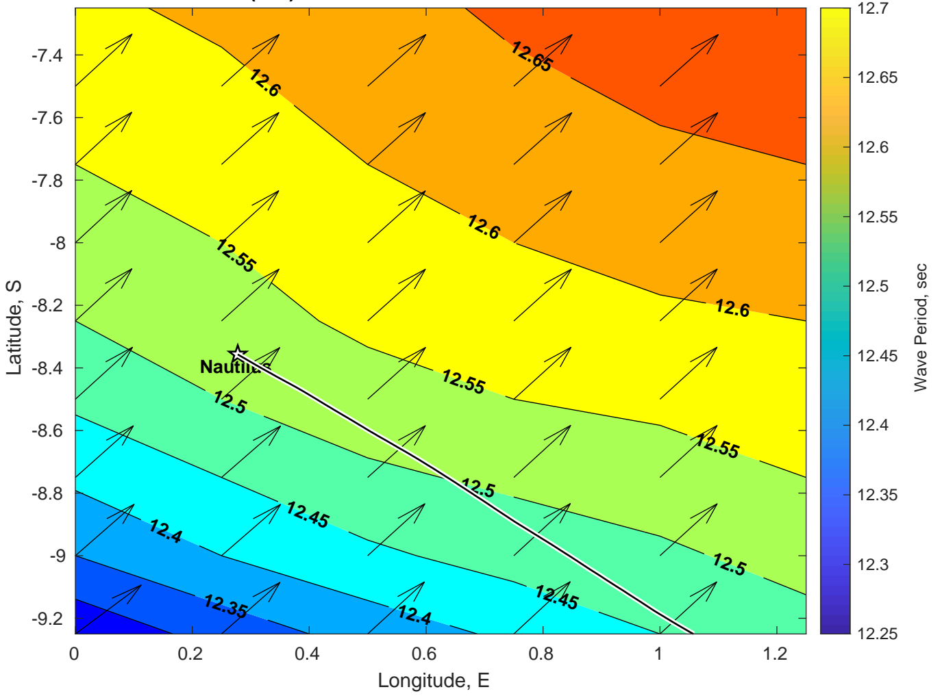
Wave Period (sec) for Nautilus at 19-Mar-2025 21:00:00
