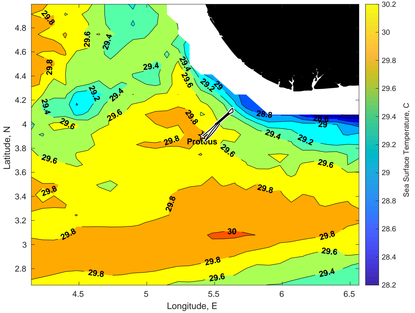
SST for Proteus at 19-Mar-2025 00:00:00
