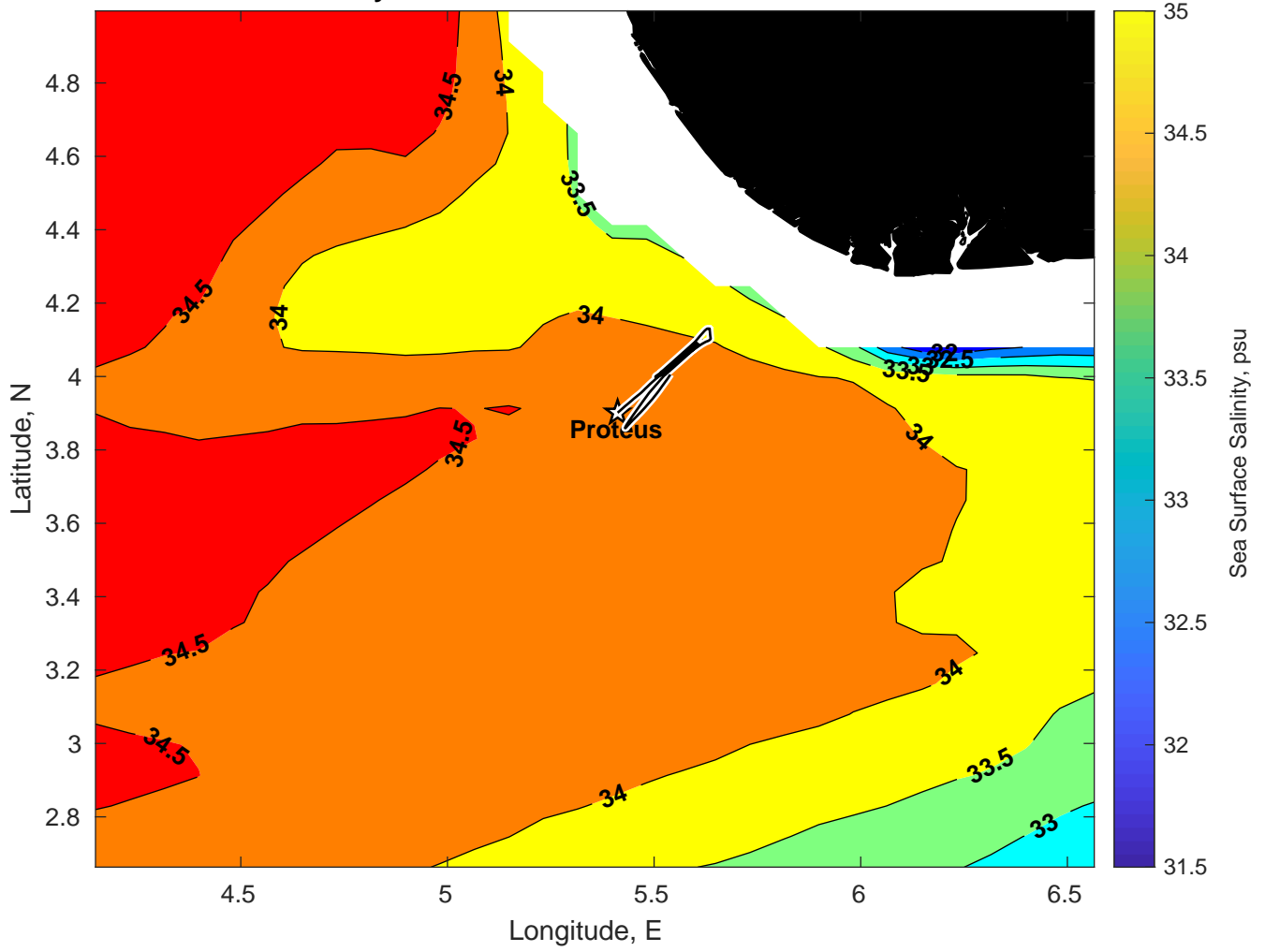
Surface Salinity for Proteus at 19-Mar-2025 00:00:00
