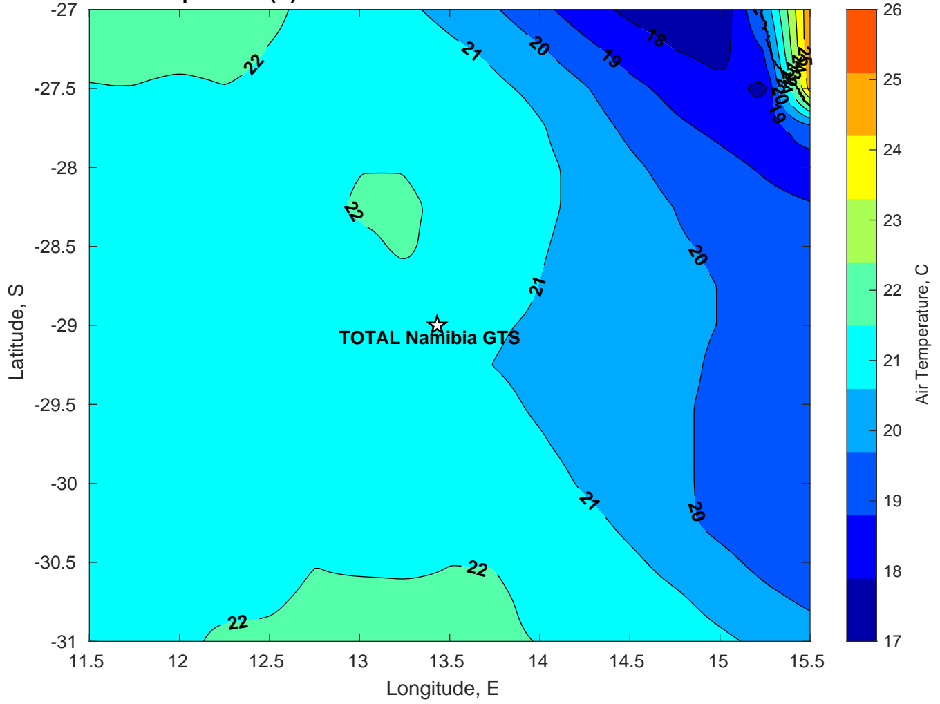
Air Temperature (C) for TOTAL Namibia GTS at 19-Mar-2025
