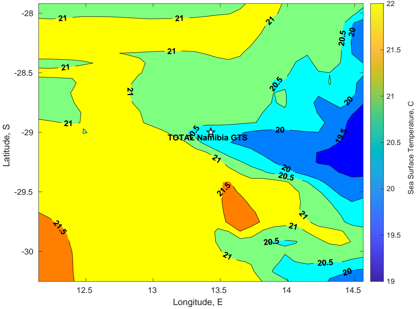
SST for TOTAL Namibia GTS at 19-Mar-2025 00:00:00
